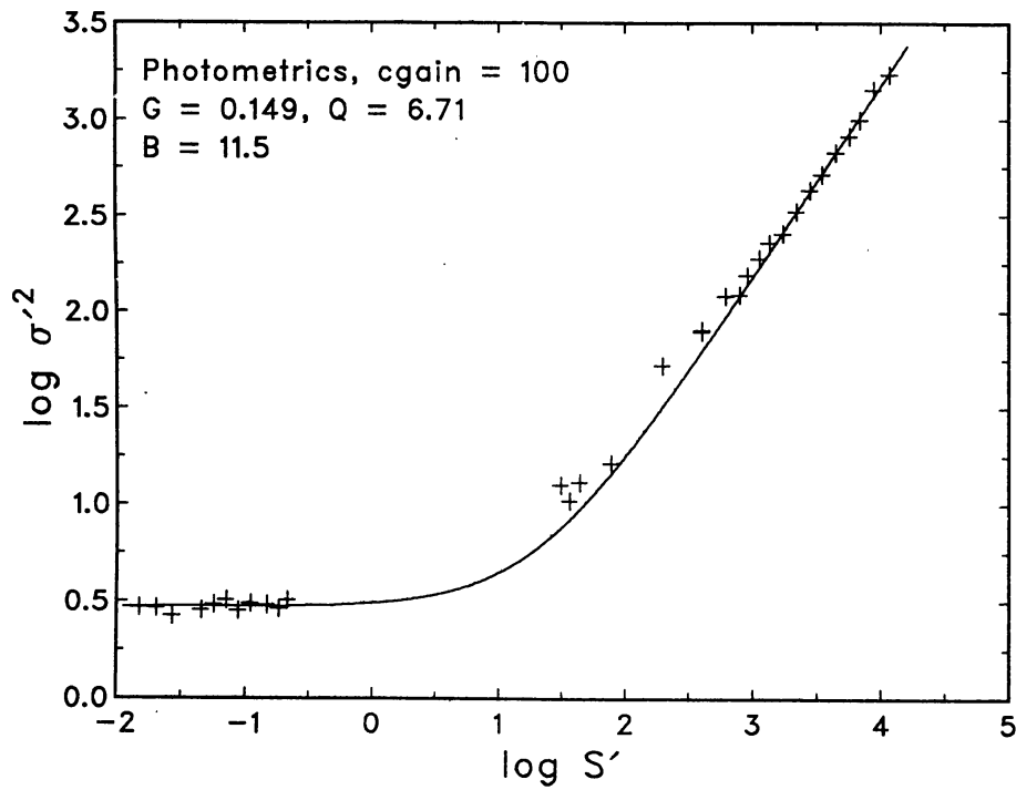
Figure 4. The logarithmic plot of variance versus signal together with the theoretical fit for the Photometrics CCD system and cgain = 100. The fit is based on data in the range S > 600 , and the bias statistics. Other details are as in Fig. 1.
