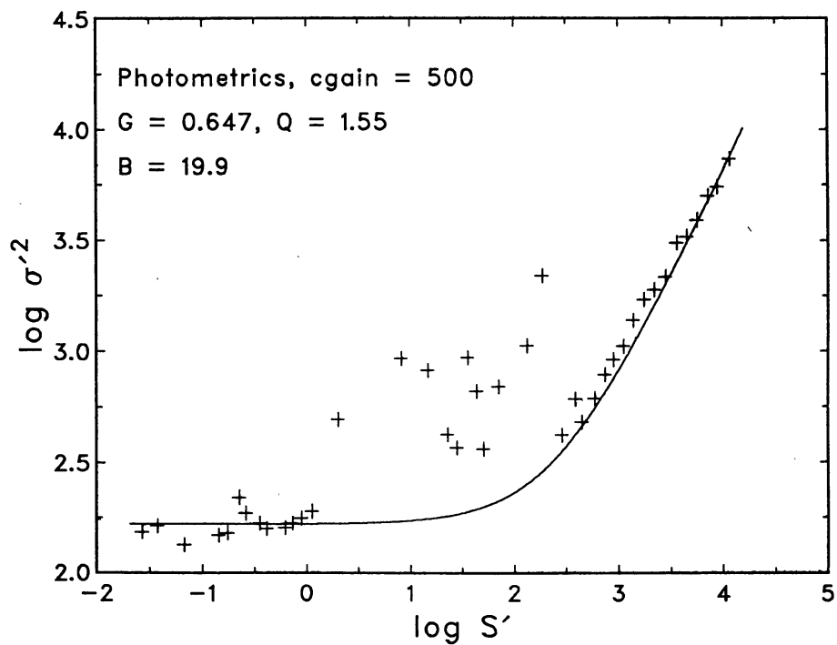
Figure 5. The logarithmic plot of variance versus signal together with the theoretical fit for the Photometrics CCD system and cgain = 500. The fit is based on data in the range S > 3000 , and the bias statistics. Other details are as in Fig. 1. Note the discordant data for S = 1 - 100 counts (1 - 150 electrons), which is probably due to the low-level charge transfer inefficiency (the 'deferred charge' problem).
