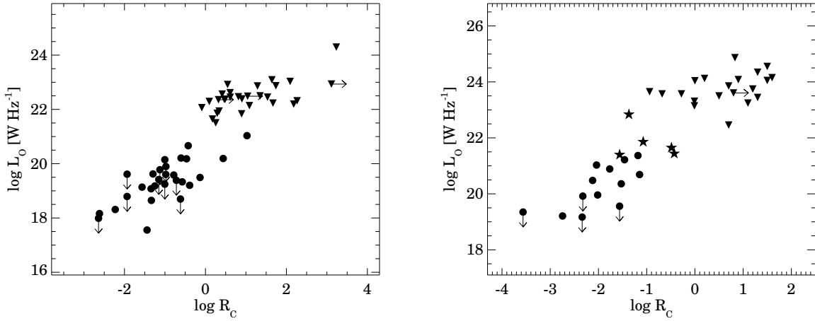
Fig. 4. Nuclear optical luminosity L_o versus radio core prominence R_c for the matched subsample of FRI galaxies and BL Lac objects (left) and FR II galaxies and quasars (right). • radio galaxies, ▼ BL Lac objects (left) and quasars (right), ★ BLRGs, ↓ upper limits, → lower limits. Statistics for the fits are listed in Table 1.
