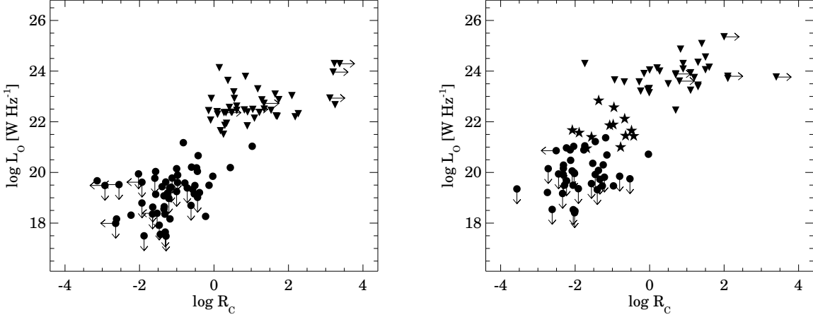
Fig. 3. Nuclear optical luminosity L_o versus radio core prominence R_c for the FRI population (left) : • radio galaxies, ▾ BL Lac objects. L_o vs. R_c for the FRII population (right) : • radio galaxies, ▾ radio-loud quasars, ★ BLRGs. ↓ and ← upper limits, → lower limits. Statistics for the fits are listed in Table 1.
