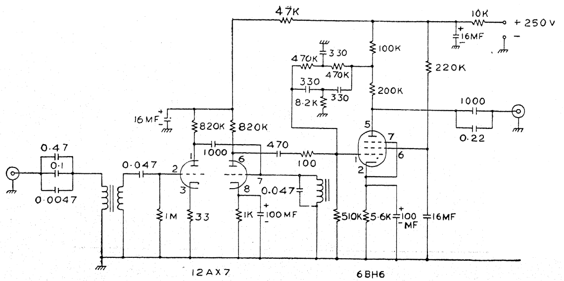
Fig. 4. Preamplifier
