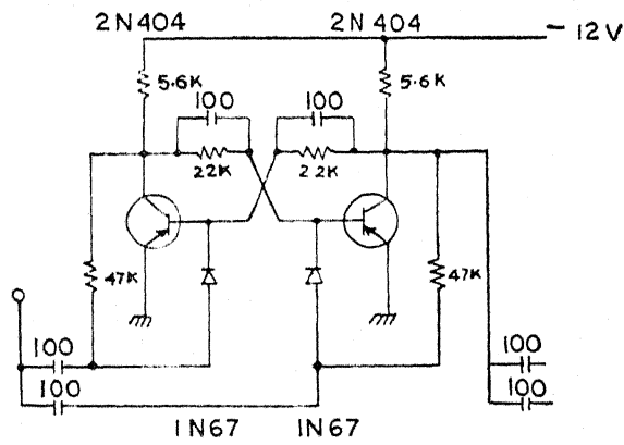
Fig. 6. Binary Divider
