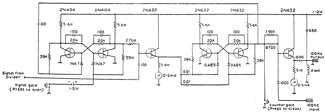
Fig. 7. Gating circuits
