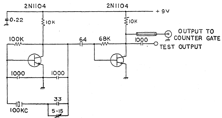
Fig. 8. 100 Kc/s oscillator
