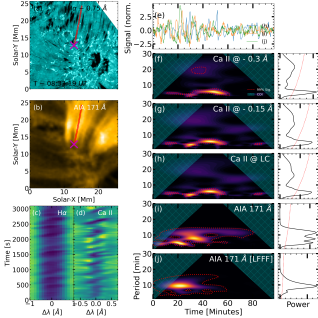
Figure 10. Similar to Figure 2 and also indicated by the blue magnetic field line in Figure 13.
