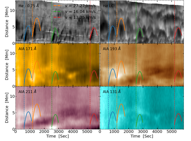
Figure 11. Same as Figure 3, but for the slit location shown in Figure 9.
