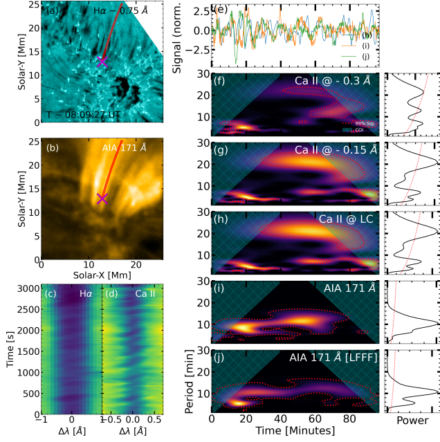
Figure 9. Similar to Figure 2 and also indicated by the green magnetic field line in Figure 13.
