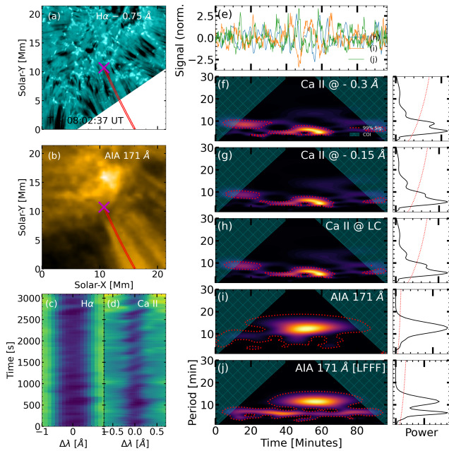
Figure 2. Panels (a) and (b) show the chromospheric and the low coronal structures of the solar atmosphere as observed in the blue wing of H \alpha and AIA 171 Å, respectively. Panels (c) and (d) present the \lambda - t diagrams of the H \alpha and Ca II 8542 Å spectral lines at the location marked by the cross (X) in panel (a). The red slit (or box) in panels (a) and (b) indicates the region used to construct the x - t map shown in Figure 3. Panel (e) shows the time series of the normalized Doppler signals of the Ca II 8542 Å line center and AIA 171 Å light curves only for clarity. Panels (f)–(h) display the wavelet analysis of the Ca II 8542 Å Doppler velocity time series (indicated in panel (e)), obtained at multiple heights at the shock wave locations covering lower to upper chromosphere, whereas panel (i) presents the wavelet analysis of the corresponding AIA 171 Å light curve (shown in panel (e)). Panel (j) also presents the wavelet analysis of the AIA 171 Å light curve, but for the location obtained from the LFFF extrapolation, as indicated by the red magnetic field line in Figure 13.
