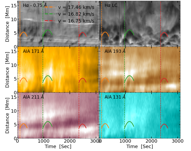
Figure 12. Same as Figure 3, but for the slit location shown in Figure 10.
