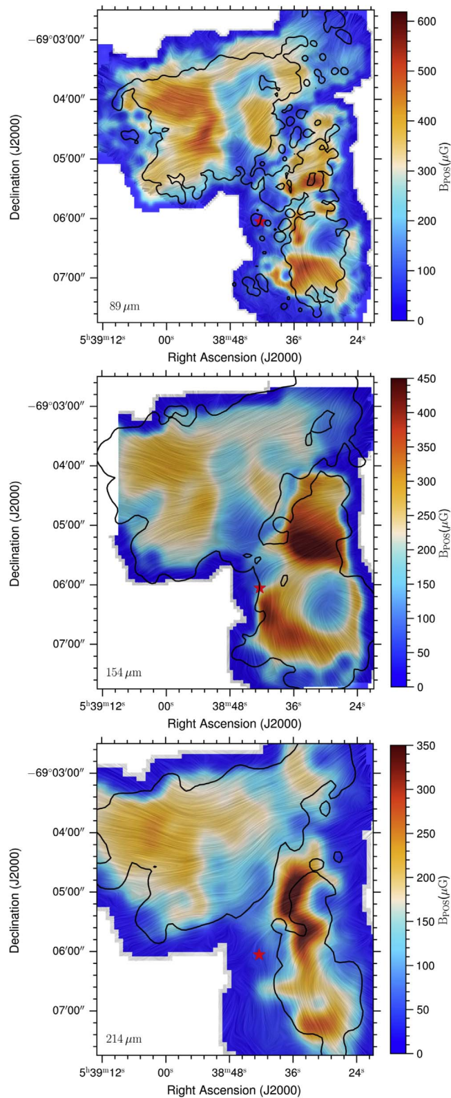
Figure 10. Maps of B_{POS} strength for all three bands (from top to bottom) using [C II] overlaid with the B -field orientation. The black contours indicate the region where I/\sigma_I \geq 100 , and p/\sigma_p \geq 3 . The star symbol indicates the R136 location. The B -field strength is weaker at longer wavelengths with peaks offset from the total intensity.
