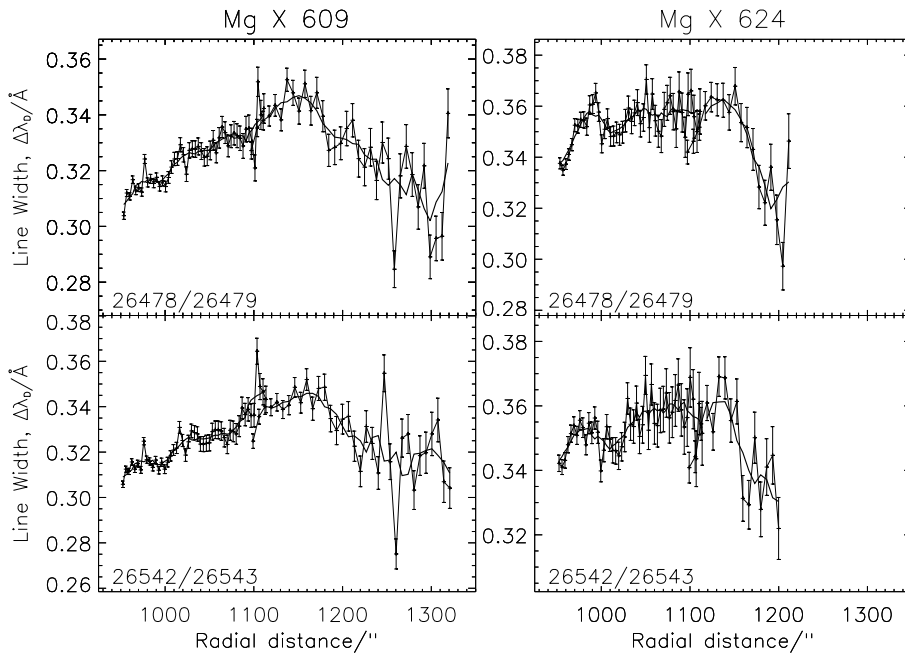
Fig. 2. Variation of the Doppler width (uncorrected for instrumental width contributions) versus radial distance for the 26 478/26 479 and 26 542/26 543 datasets, as indicated by the numbers shown in each plot. The thick black lines show the result of a box-car averaging to remove the effects of the FPN. Radial distance locations where the radiance fell below a critical S/N value do not show the results of the line width measurements.
