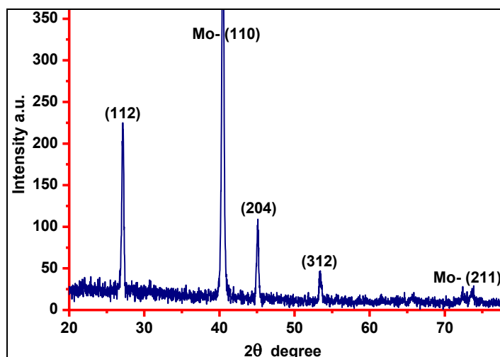
Fig. 1 X-ray diffraction of CZTS/Mo/SLG thin film layers
