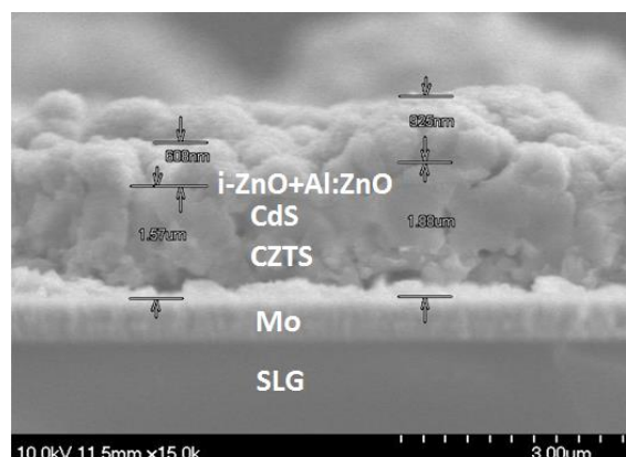
Fig. 3 SEM cross section of our Al:ZnO/i-ZnO/ZnCdS/CZTSe/Mo/SLG device structure
