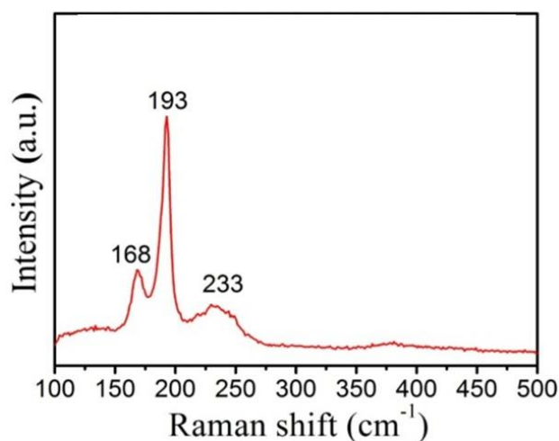
Fig. 4 Raman spectrum of the fabricated CZTS absorber layer
