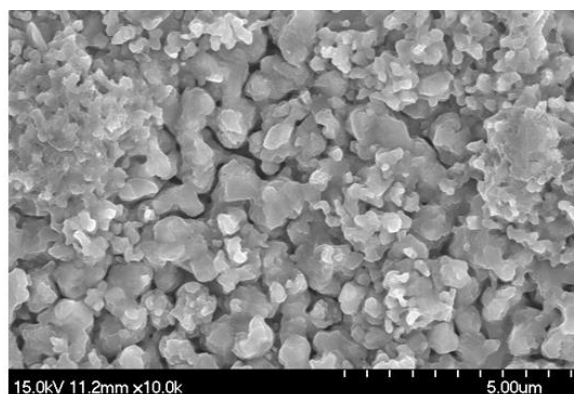
Fig.2 SEM top surface morphology of the fabricated CZTSe thin film absorber layer
