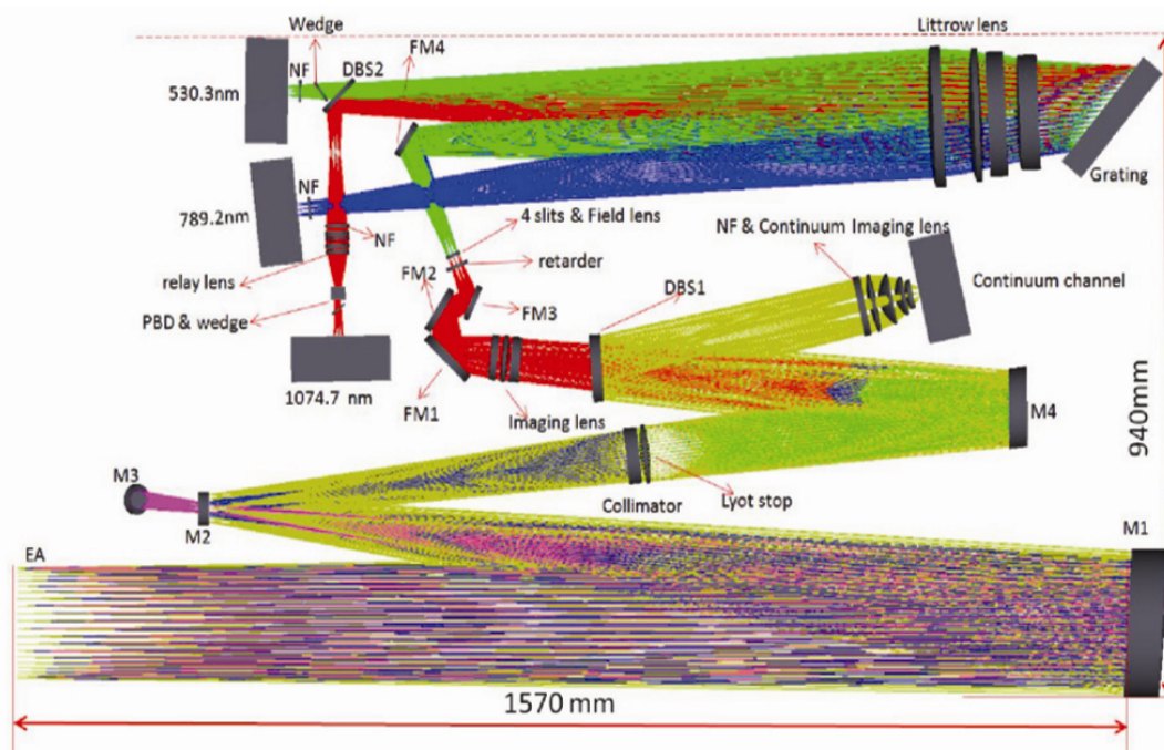
Figure 1. Optical layout of Visible Emission Line Coronagraph (VELC).
