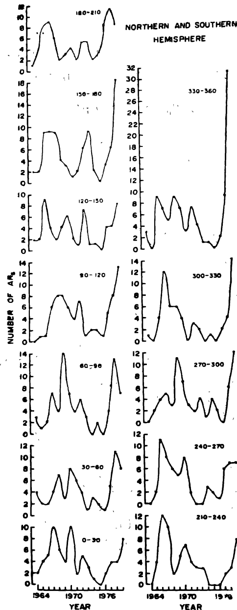
Figure 4. The number of high flare-activity active regions for each longitude strip of 30°-wide range as a function of time.
