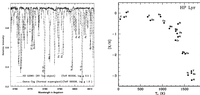
Figure 1. The left panel shows the spectrum of HD 52961 compared with a standard star of very similar temperature and gravity. The dependence of elemental depletion on T_C is illustrated in the right panel for HP Lyr.
