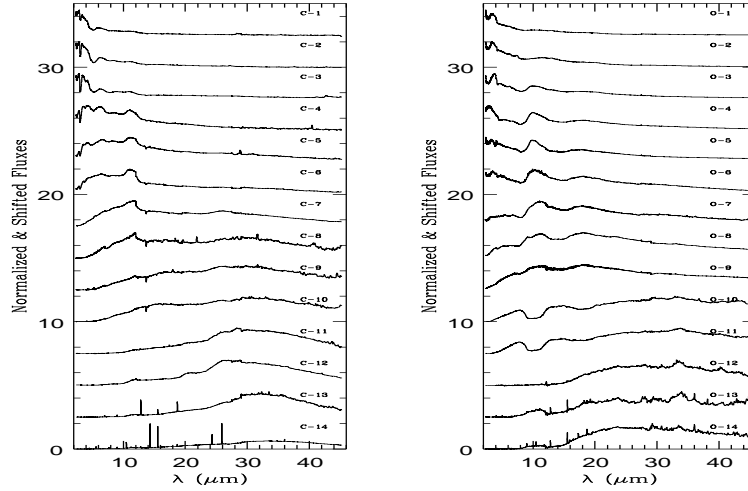
Figure 2. The evolutionary sequence as inferred from the IR spectra. The left panel shows C-rich sources and the right O-rich ones (Figure courtesy P. García-Lario, reproduced from proc. IAUS, 234, 397 eds M. J. Barlow & R. H. Méndez, by permission of Cambridge Univ Press)
