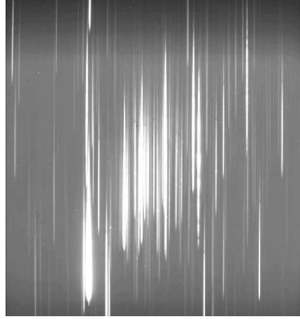
Figure 1. The slitless spectral image of NGC 7419.
