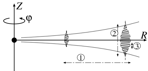
Fig. 1 The mode structure with three different scale lengths.
