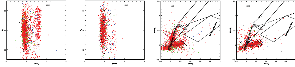
Figure 1. CMDs ((B-V)_0 vs V_0 ) and CCDs ((H-K)_0 vs (J-H)_0 ) for the cross matched stars in the LMC and SMC
