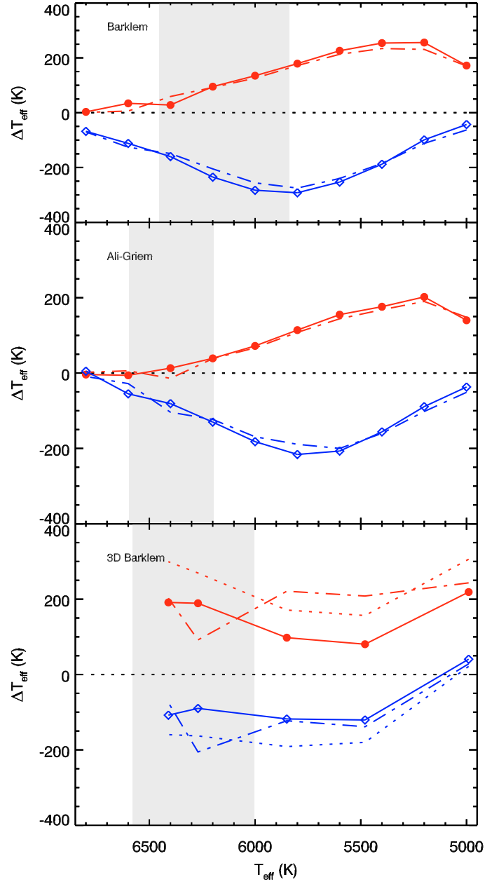
Fig. 3. H\alpha theoretical profiles for models with \log g = 4 , [\text{Fe}/\text{H}] = -3 (solid lines) and \log g = 4 , [\text{Fe}/\text{H}] = -2.5 (dot-dashed lines) have been fitted with the same procedure used for the program stars, but using a \log g = 3.5 grid (red lines with filled circles) and a \log g = 4.5 grid (blue lines with open diamonds). Here we plot the temperature difference ( T_{\text{eff}}(\log g = 3.5/4.5) - T_{\text{eff}}(\log g = 4.0) ), against the “real” effective temperature of the profile. The upper panel shows BA profiles, the middle panel ALI profiles, and lower panel 3D profiles. The gray shaded areas indicates the temperature ranges for the program stars in each T_{\text{eff}} scale.
