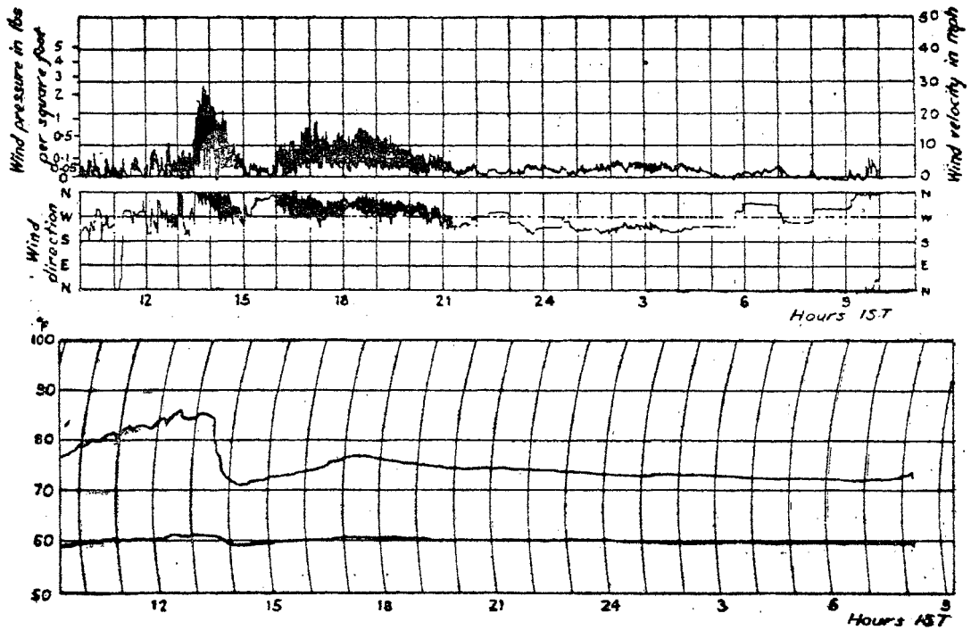
Fig. 15. Dines P.T. Anemogram (19-20 September 1937) with the corresponding thermogram chart
