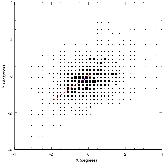
Fig. 1. Number density distribution of RR Lyrae stars in the LMC. The optical center is shown as red cross, the center of the RRLS density is shown in blue cross, the PA_{maj} is shown in red line.
