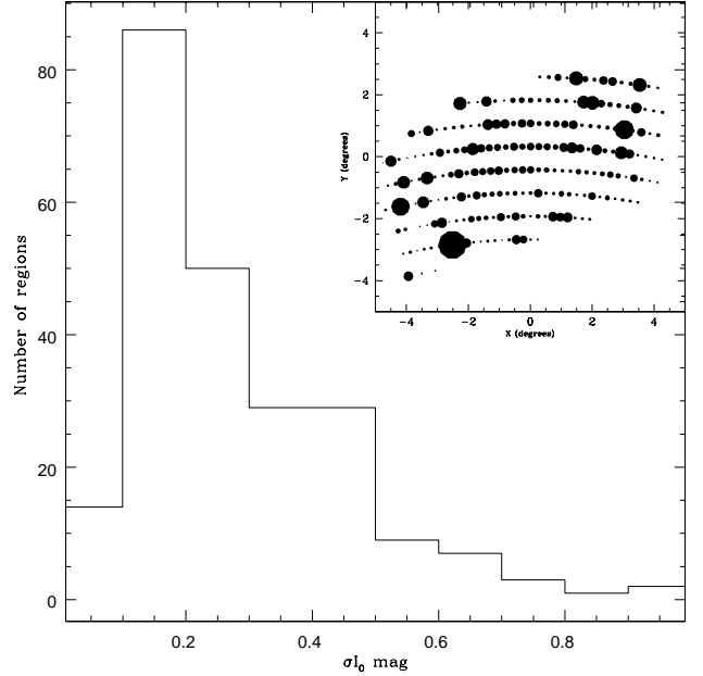
Fig. 3. The histogram of the dispersion in RRLS ( \sigma I_0 ). The figure in the inset shows the X-Y location of the bins, where the size of the points is proportional to the dispersion.
