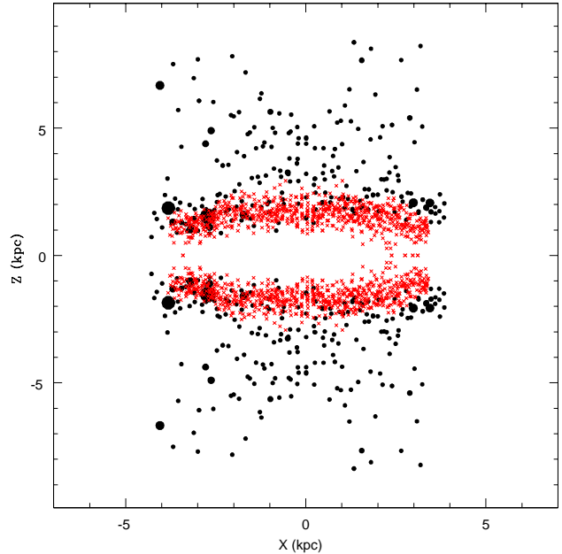
Fig. 2. The distribution of scale-height of ab type RRLS (black) compared with that of RC stars (red). The scale heights shown are the dispersion in the mean magnitude reflected about z=0 . The larger sized dots indicate larger error in the estimated dispersion.
