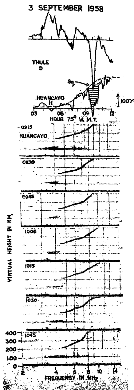
Fig. 4. Ionograms at Huancayo during the DP 2 sub-storms on 3 September 1958 inhibiting the occurrence of E s at 0945 to 1015 hr.
