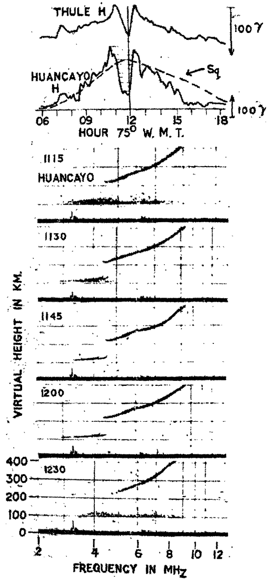
FIG. 3. Magnetograms at Huancayo during a DP_2 type polar sub-storm on 18 March 1958. Note the disappearance of E_s between 1130-1200 hrs during the depression in H at Huancayo.
