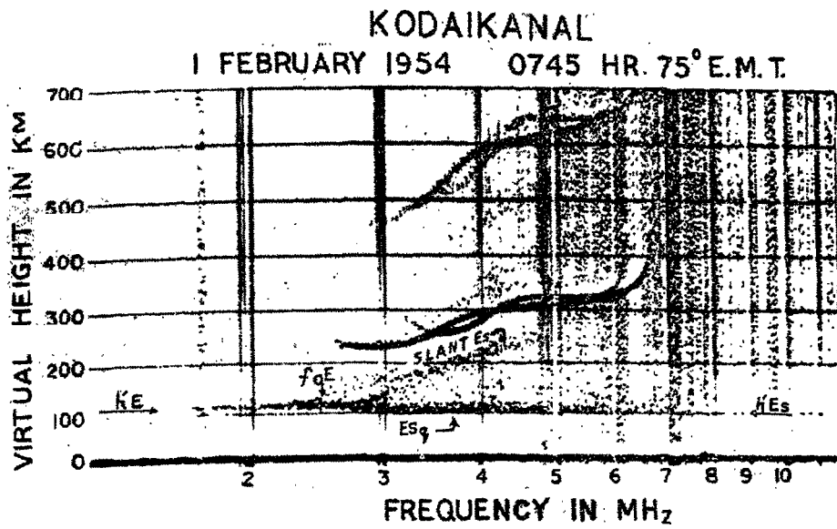
FIG. 1. An ionogram taken at Kodaikanal showing the q and s (slant) types of sporadic E, f_0 E , h' E and h' E_s .
