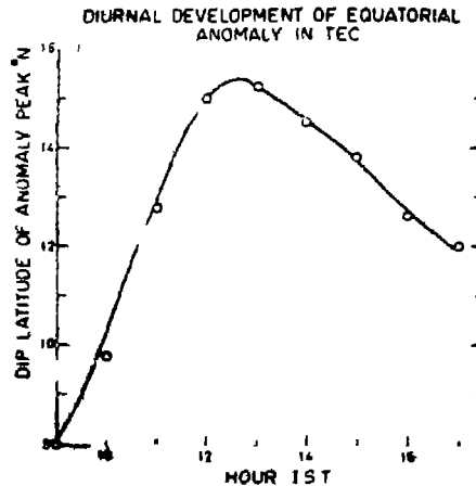
Figure 3. Diurnal development of the equatorial anomaly in TEC depicted by the movement of the dip latitude of the peak of the anomaly
