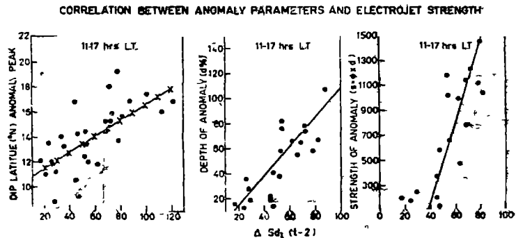
Figure 5. Variation of the dip latitude, \phi , of the anomaly peak (left), the normalized depth, d (middle), and the strength, S = \phi \times d (right) of the anomaly with equatorial electrojet strength two hours prior to the anomaly.
