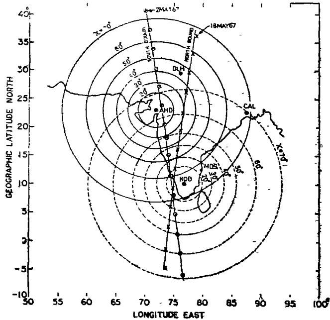
Figure 1. Contours of constant zenith angles for a satellite at 1000 km as observed from Ahmedabad (full lines) and Kodakanel (dashed lines). Two typical sub-satellite tracks, one for 18 May 1967 (North-bound) and the other for 2 May 1967 (South-bound) are also shown to indicate the region of coverage when observed from both the stations.
