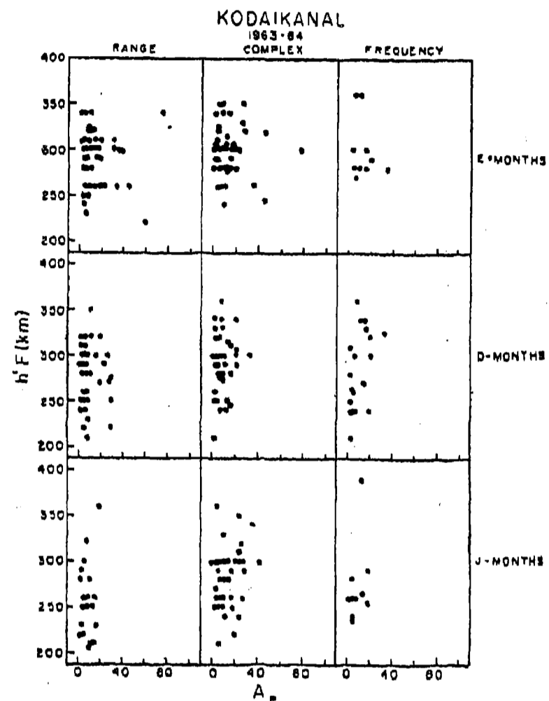
FIG. 1. Mass plots of h'F corresponding to the first post sunset appearance of spread-F at Kodaikanal during the period: January 1963-December 1964.
