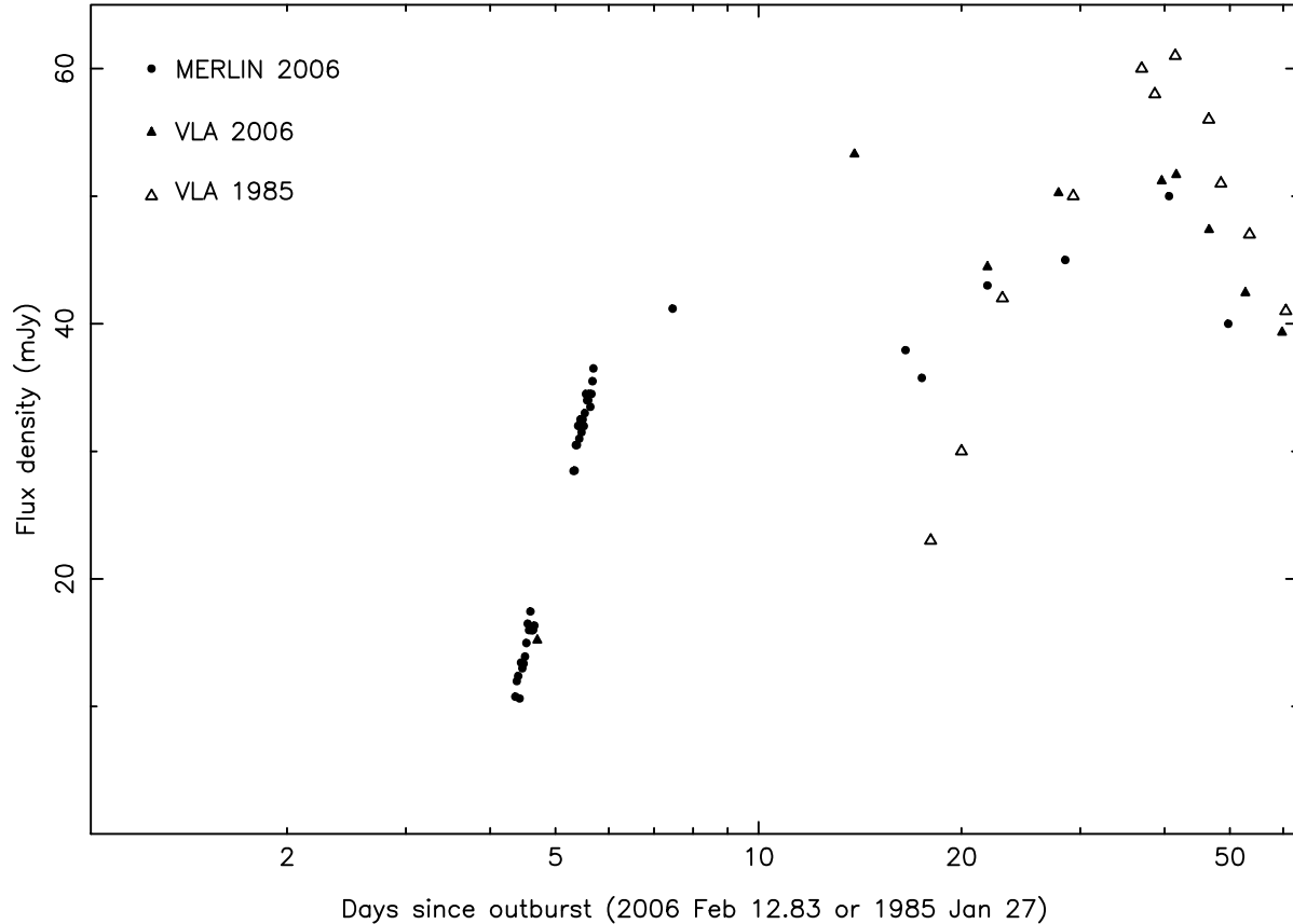
Figure 1. Radio lightcurves at 5 to 6 GHz. Symbols: 2006 VLA=filled triangles; MERLIN=filled circles (small ones during the initial rise – error bars not included); 1985 VLA open triangles – observations during the 1985 outburst from Hjellming et al. (1986). Uncertainties are smaller than or comparable to the symbol size except where error bars indicate otherwise.
