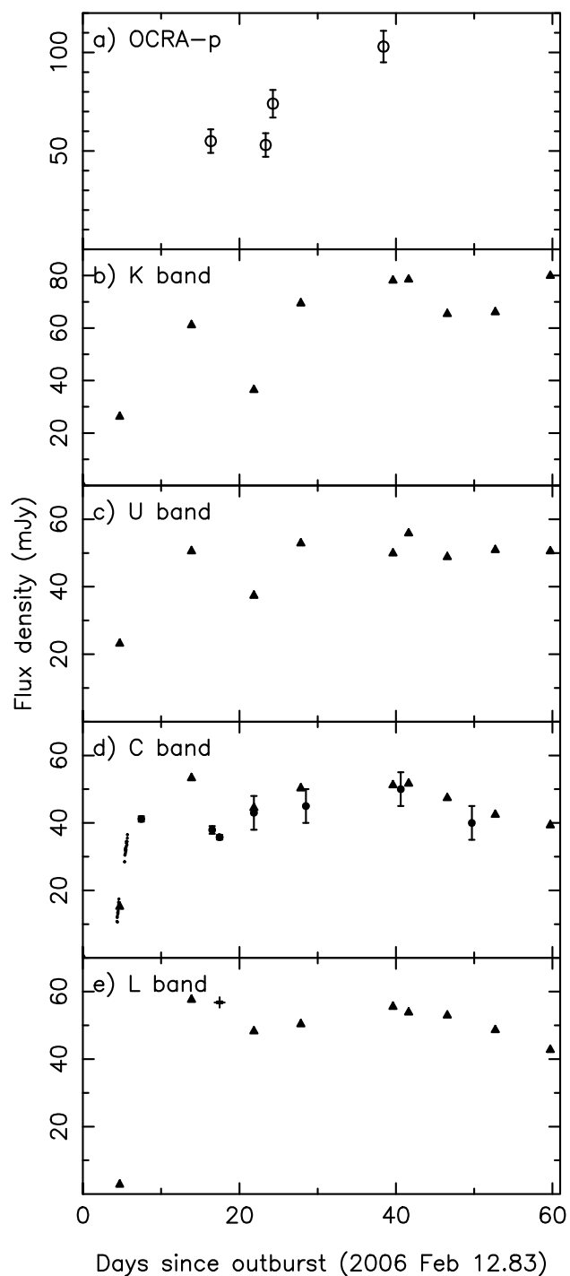
Figure 2. Radio lightcurves at different frequencies. (a) 30 GHz with OCRA-p. (b) K band – 22.48 GHz with the VLA. (c) U band – 14.96 GHz with the VLA. (d) For comparison: C band – 4.88 GHz with the VLA, 6 GHz with MERLIN. (e) L band – 1.46 GHz with the VLA, 1.39 GHz with the GMRT and 1.66 GHz with MERLIN. Symbols: VLA=filled triangles; MERLIN=filled circles (small ones during the initial rise – error bars not included); GMRT=crosses; OCRA-p=open circles. Uncertainties are smaller than or comparable to the symbol size except where error bars indicate otherwise.
