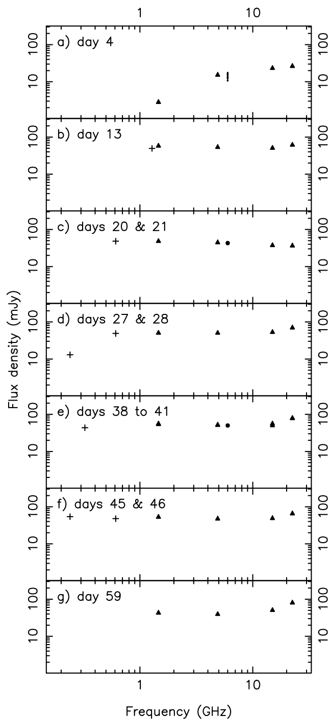
Figure 3. Radio spectrum on various days as marked. Symbols and uncertainties as Fig 2. Where available 240, 325 or 610 MHz points (crosses) from Kantharia et al. (2007) are included, demonstrating the development of emission at lower frequencies.
