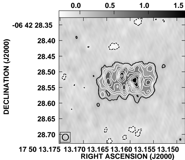
Figure 4. VLBA image at 1.667 GHz taken on day 63. Beam size is indicated in the bottom left. Greyscale range is -0.302 to 1.532 \text{mJy beam}^{-1} . Contours are at intervals of 10% of the peak of 1.532 \text{mJy beam}^{-1} ; negative contours indicated with broken lines.
