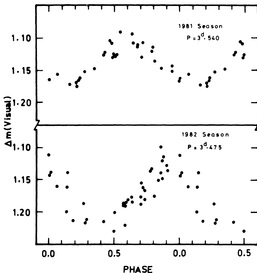
Fig. 1. Light curves of BD +25°2511 obtained during the 1981 and 1982 seasons.
