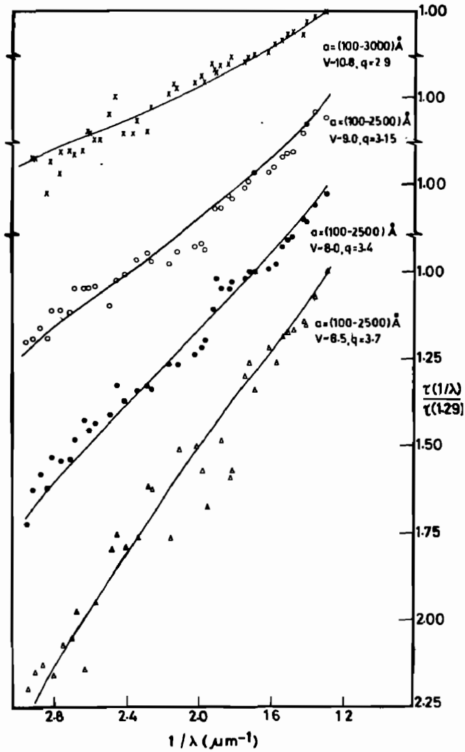
Fig-2. Extinction curves normalised at \lambda 7760 \text{ \AA} compared with theoretical ones computed for MRN size distribution. Crosses: 1 Feb. 1974, open circles; 3 June 1972, filled circles 12 June 1974, and open triangles: 10 July 1972.
