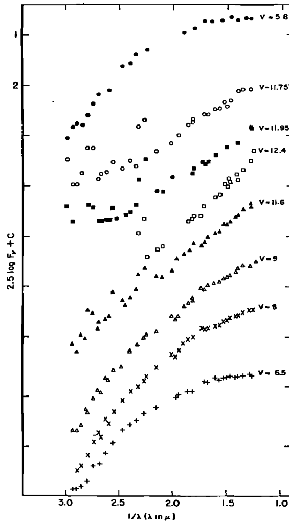
Fig. 1. 1972 minimum observations of R CrB using 36 inch crossley reflector. Pass band: 16A shortward of 5200A and 20A longward of 5200A.
