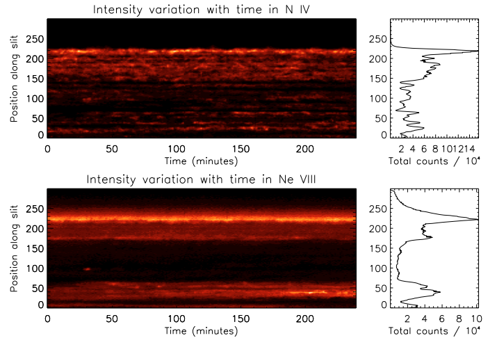
Fig. 2. Top (bottom) left panel shows the variation of the N IV 765 Å (Ne VIII 770 Å) intensity along the slit (in pixel units) with time. Right panel shows the variation of the total summed counts over time along the slit.
