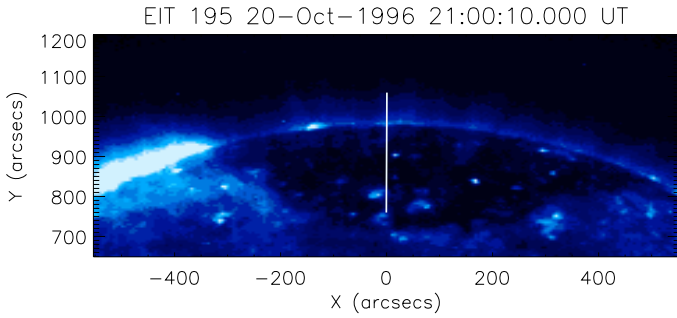
Fig. 1. Solar polar coronal holes imaged by EIT/SoHO in the 195 Å band. The vertical white lines show the fixed position of the SUMER slit.
