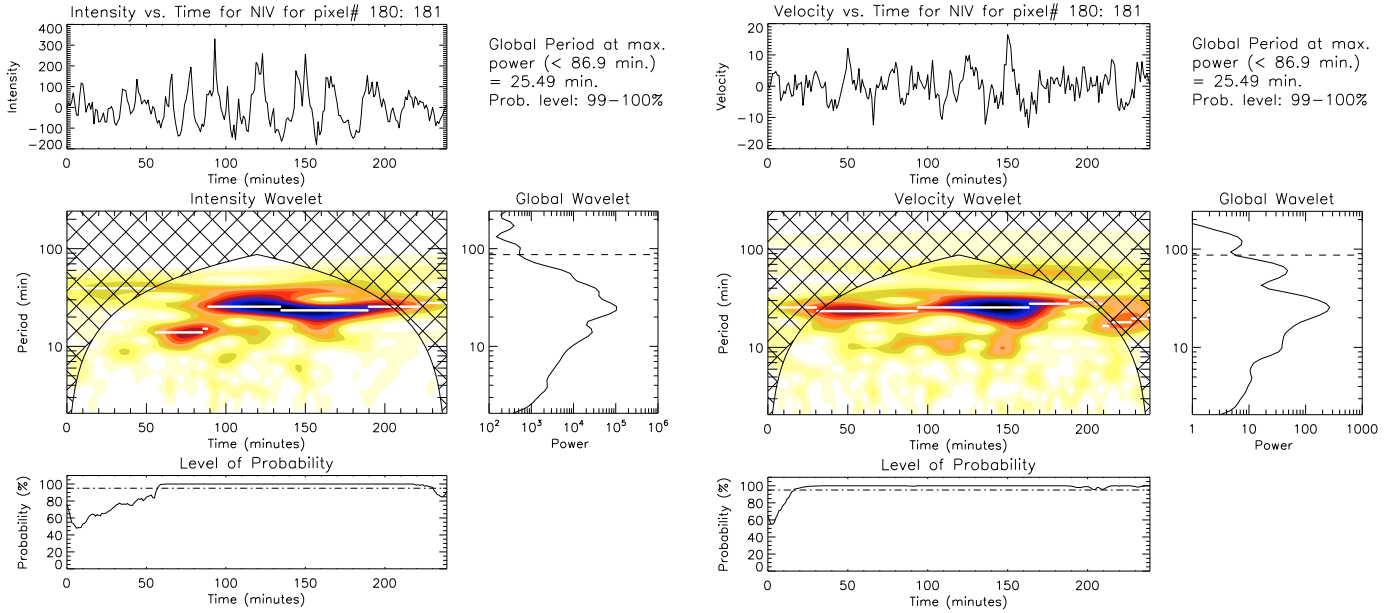
Fig. 3. The wavelet result for a bright location (pixel No. = 180–181 which corresponds to Y \approx 940'' ) in the N IV 765 Å intensity and velocity. In each set the top panels show the relative (background trend removed) radiant flux/velocity as marked, the central panels show the colour inverted wavelet power spectrum, the bottom panels show the variation of the probability estimate associated with the maximum power in the wavelet power spectrum (marked with white lines), and the right middle panels show the global (averaged over time) wavelet power spectrum. Above the global wavelet the period, measured from the maximum power from the global wavelet, together with probability estimate, is printed.
