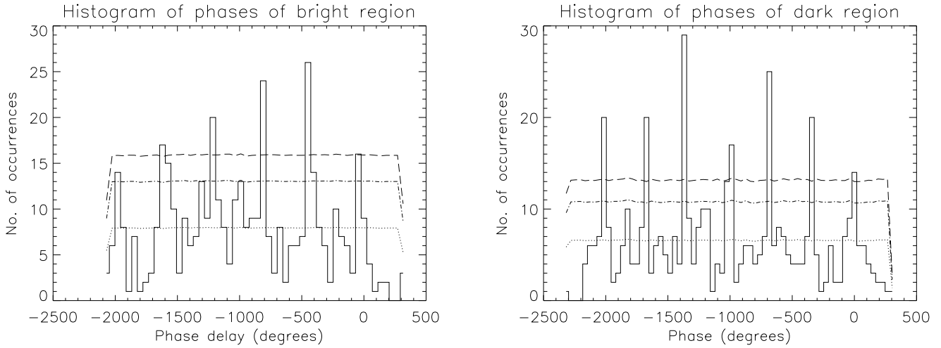
Fig. 6. Histogram showing the distribution of phase delay measurements as a function of frequency for the bright ( left panel ) and dark ( right panel ) locations for the downwardly propagating waves only. The horizontal dotted, dot-dashed and long dashed lines show the 68.3% (i.e., 1\sigma ), 90% ( \approx 1.64\sigma ) and 95% ( \approx 2\sigma ) confidence levels, respectively, calculated using Monte-Carlo simulations with 5000 permutations.
