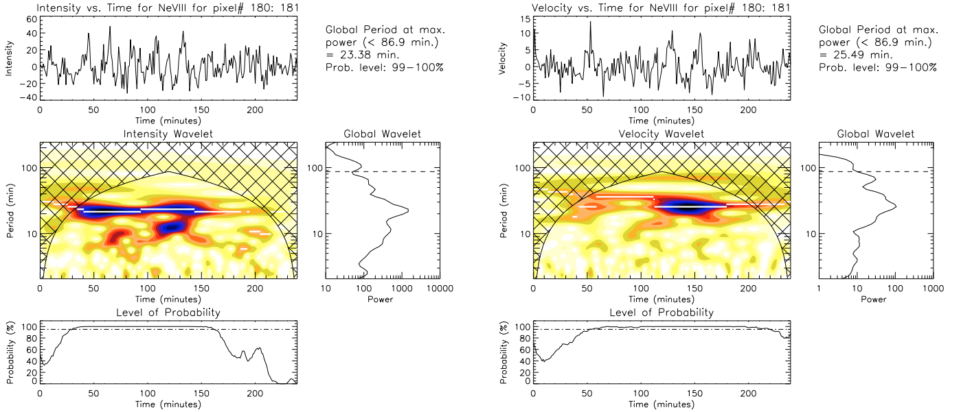
Fig. 4. The wavelet analysis results for a bright location (pixel No. = 180–181 which corresponds to Y \approx 940'' ) in the intensity (left side) and velocity (right side) data for the Ne VIII 770 Å line. The descriptions about the different panels are the same as in Fig. 3.
