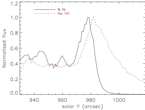
Fig. 7. Normalised flux distribution with height for the two lines. The solid line shows the distribution for N IV, while the dashed line shows the distribution for Ne VIII. The location of maximum brightness for each line is used for determining the height difference.
