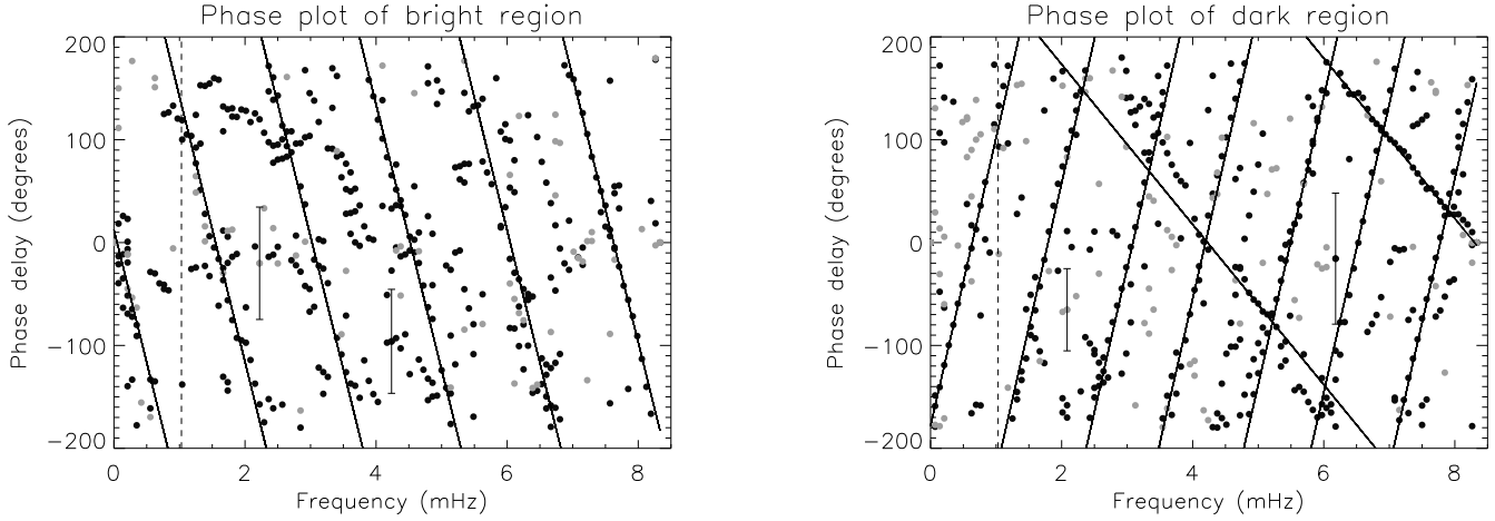
Fig. 5. Phase delays measured between the oscillations in the spectroscopic line pair for the bright ( left panel ) and dark ( right panel ) locations. The phases in radiant flux oscillations are shown in the grey circle symbols while that in LOS velocities are shown as the black circle symbols. Overplotted on each figure are black parallel lines, corresponding to fixed time delays. The vertical dashed line drawn at 1.03 mHz indicates that some phase values below this could be affected by solar rotation. Representative errors on the phase measurements are indicated by the error bars.
