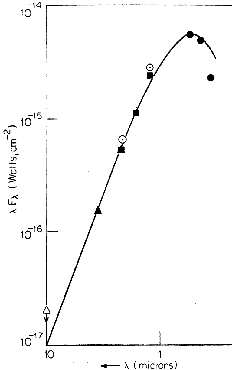
Figure 1. Energy distribution of XX Cam (Table 2) corrected for E(B-V) = 0.30 . The curve represents a black body energy distribution (full line) for 7000 K which is made to agree with the observations at 0.55 microns.
