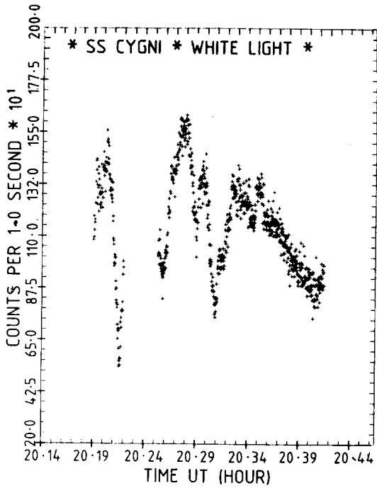
Figure 2. Unfiltered light curve of SS Cygni
