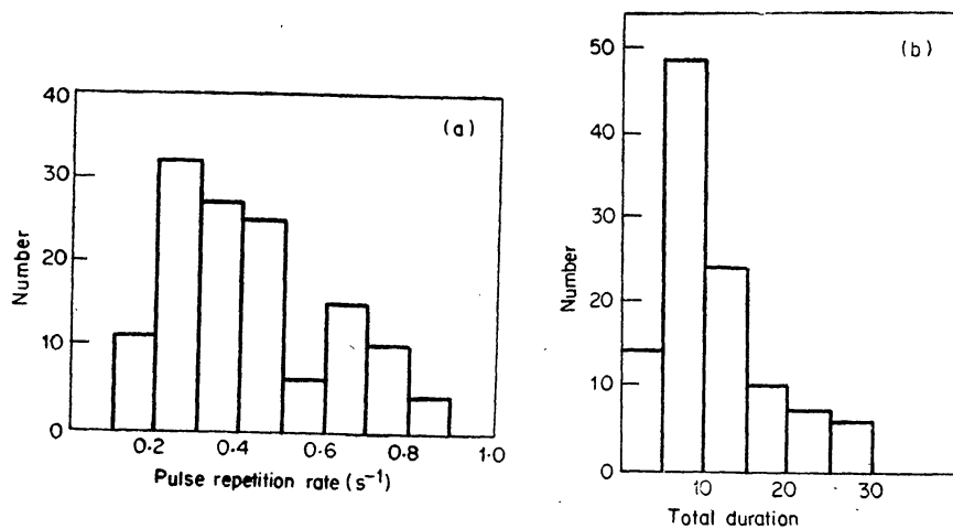
Figure 3a. Histogram of the number of bursts versus the pulse repetition rate.
