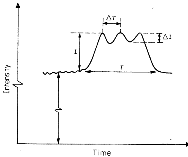
Figure 2. Explanation of the burst parameters.
