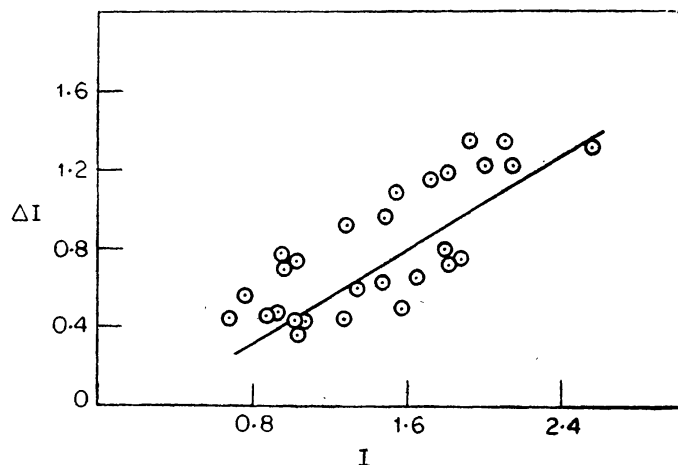
Figure 4. A plot between the average peak intensity \langle I \rangle and the average pulse amplitude \langle \Delta I \rangle shows a strong correlation between \langle I \rangle and \langle \Delta I \rangle .
