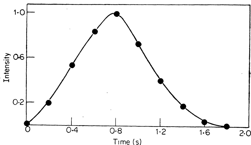
Figure 5. The average time profile of a pulse.
