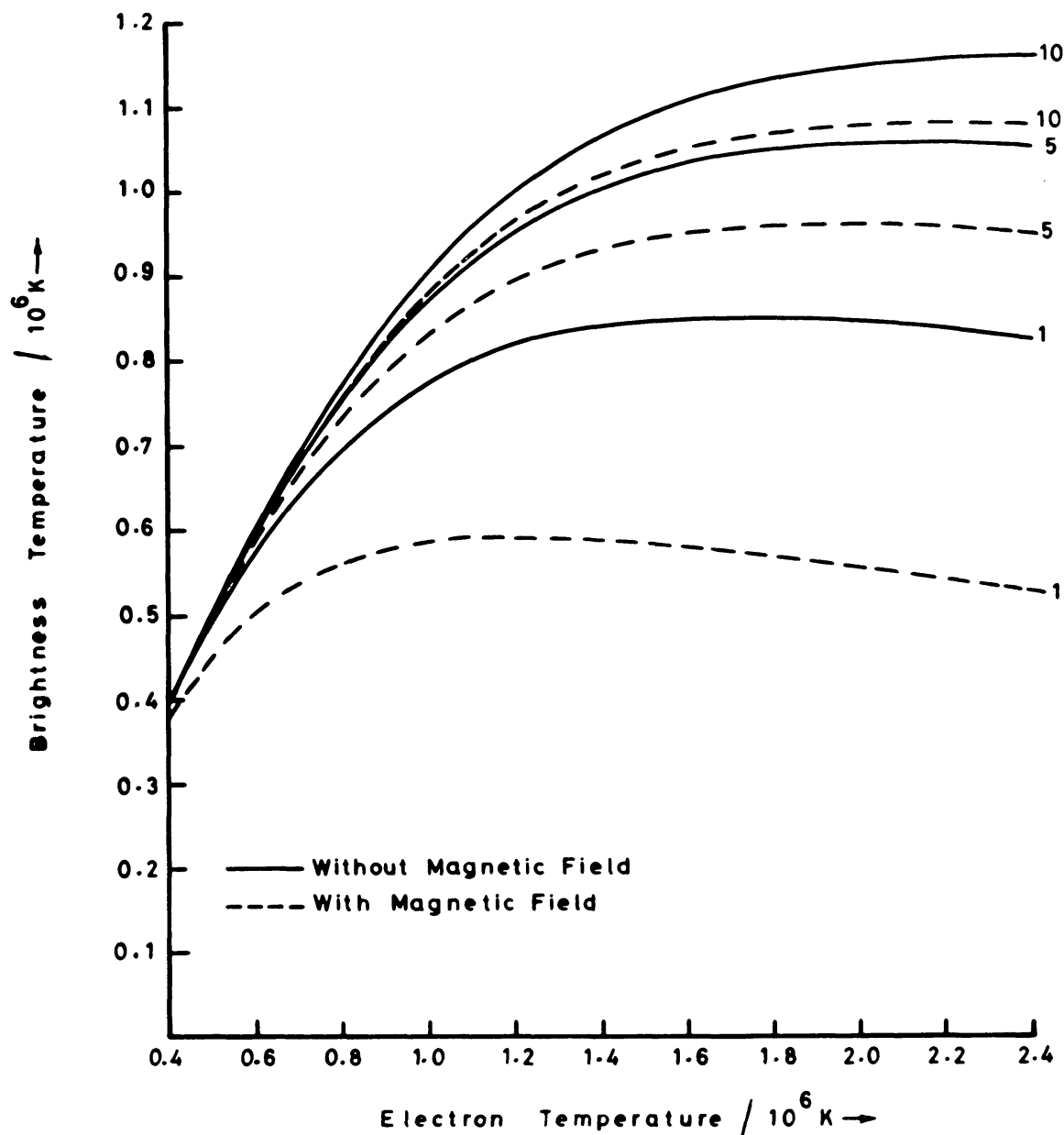
Fig. 5a. Calculated brightness temperature with magnetic field included vs electron temperature for various electron densities.
