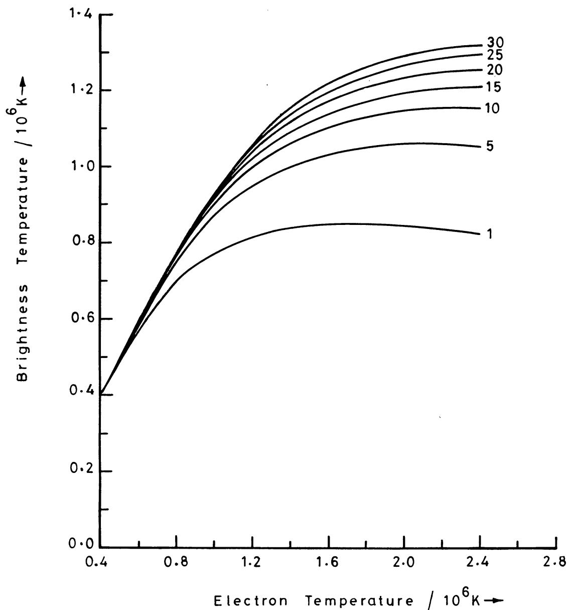
Fig. 4a. Calculated brightness temperature vs electron temperature in the corona for various electron densities.
