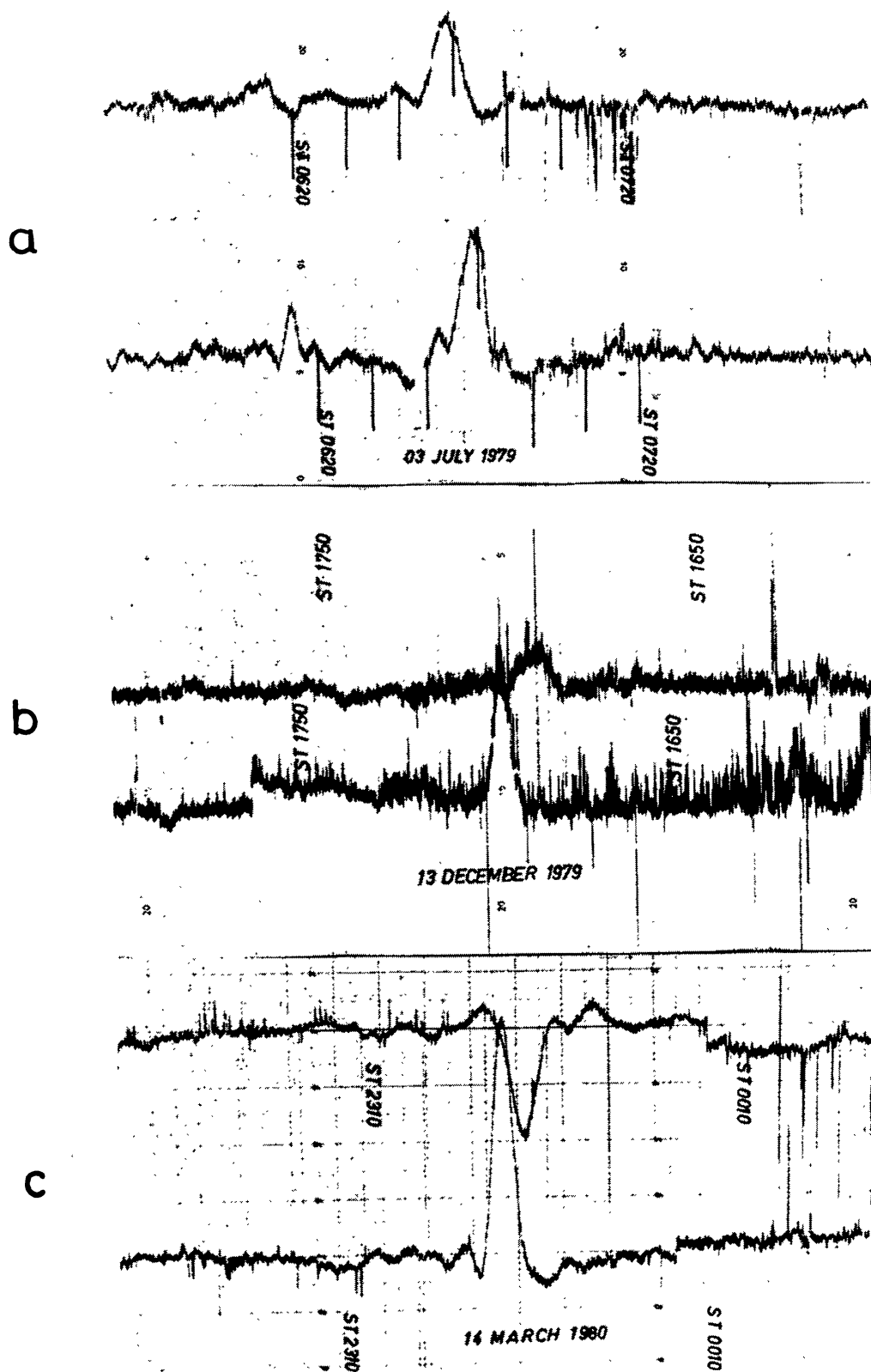
Fig. 1a-c. Typical examples of records depicting continuum radio emission from the Sun.
