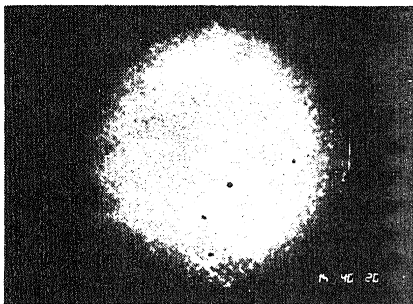
Figure 2. An example of the calcium K-line filtergram of the Sun, taken on 8 January 1990. The network pattern can be seen clearly. Also seen are other features associated with solar activity, like sunspots (dark spots) and bright emission areas surrounding sunspots, called plages.
