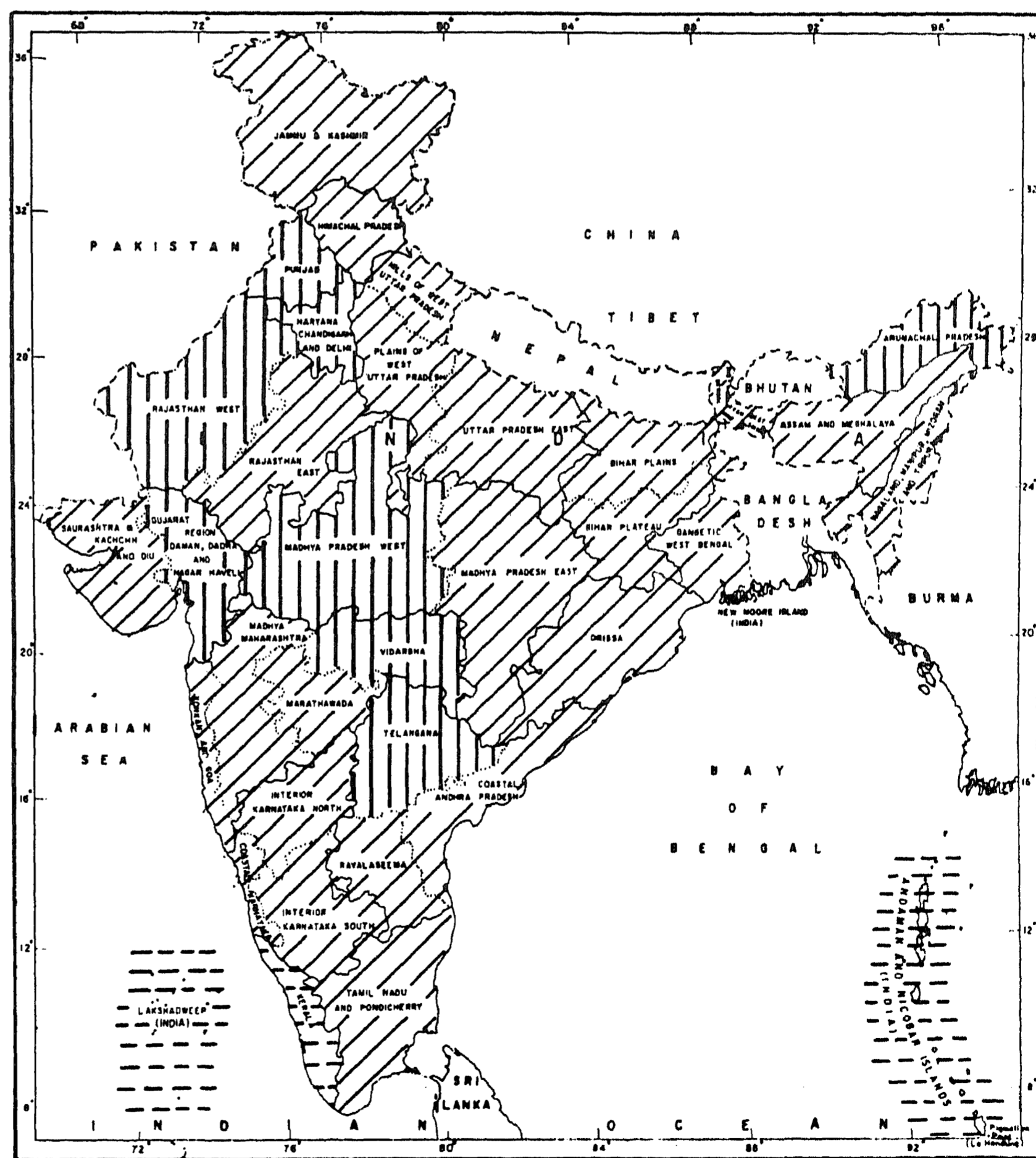
Figure 1. Cumulative rainfall for the period 1 June 1990 to 30 September 1990.
