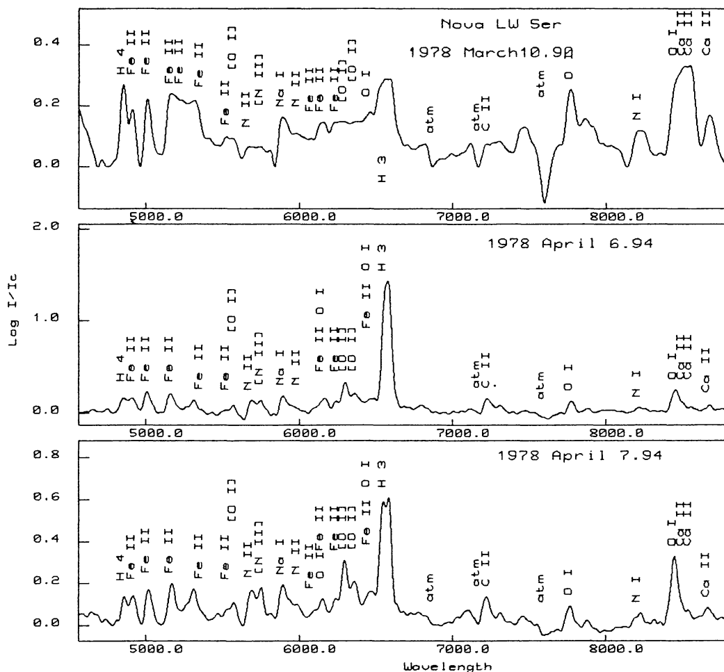
Figure 1 The spectra of LW Ser. The lines at 6300 and 6363 Å signifying the [O I] flash are evident on April 6 and 7.
