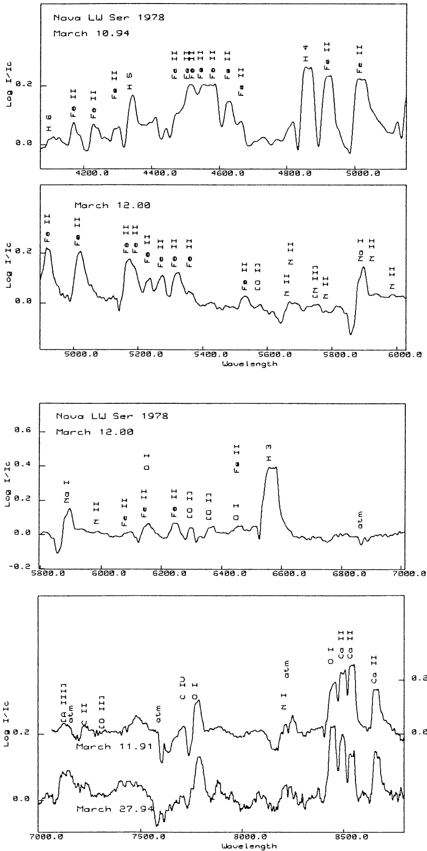
Figure 4 Spectra of LW Ser at higher resolutions.
