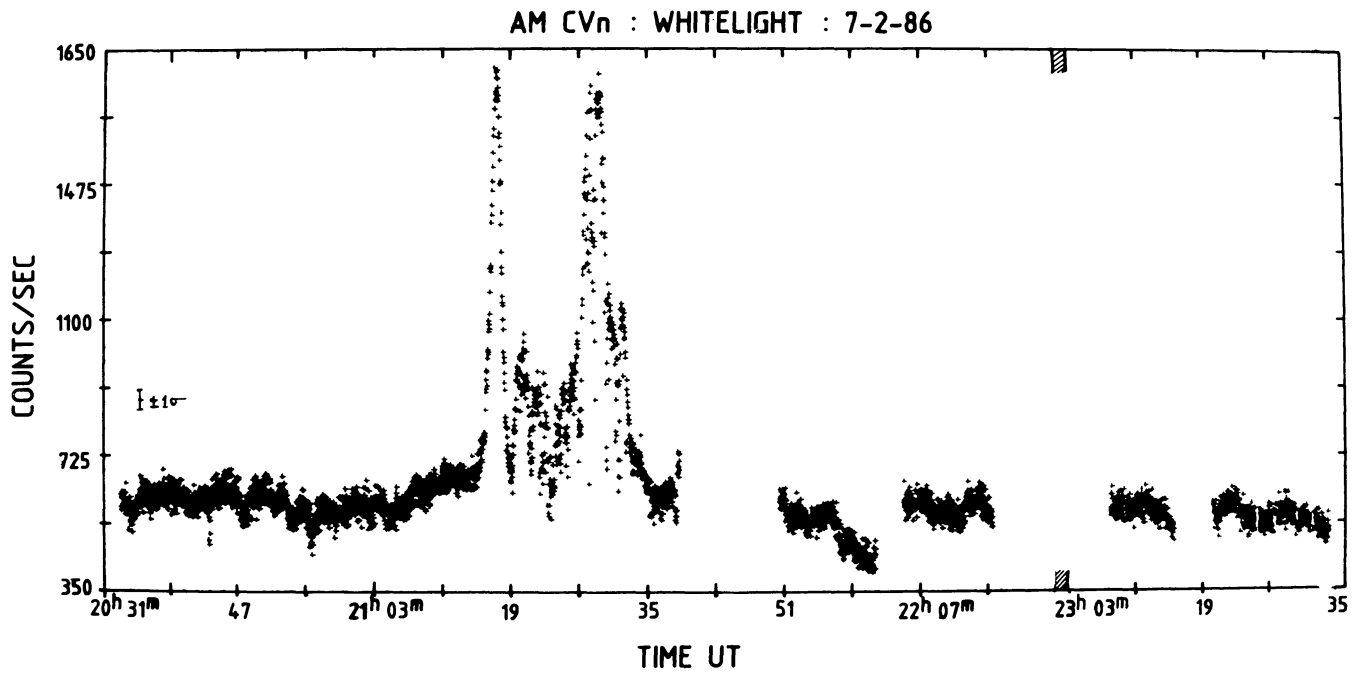
Fig. 2a. Flare of AM CVn on 1986 Feb. 7
