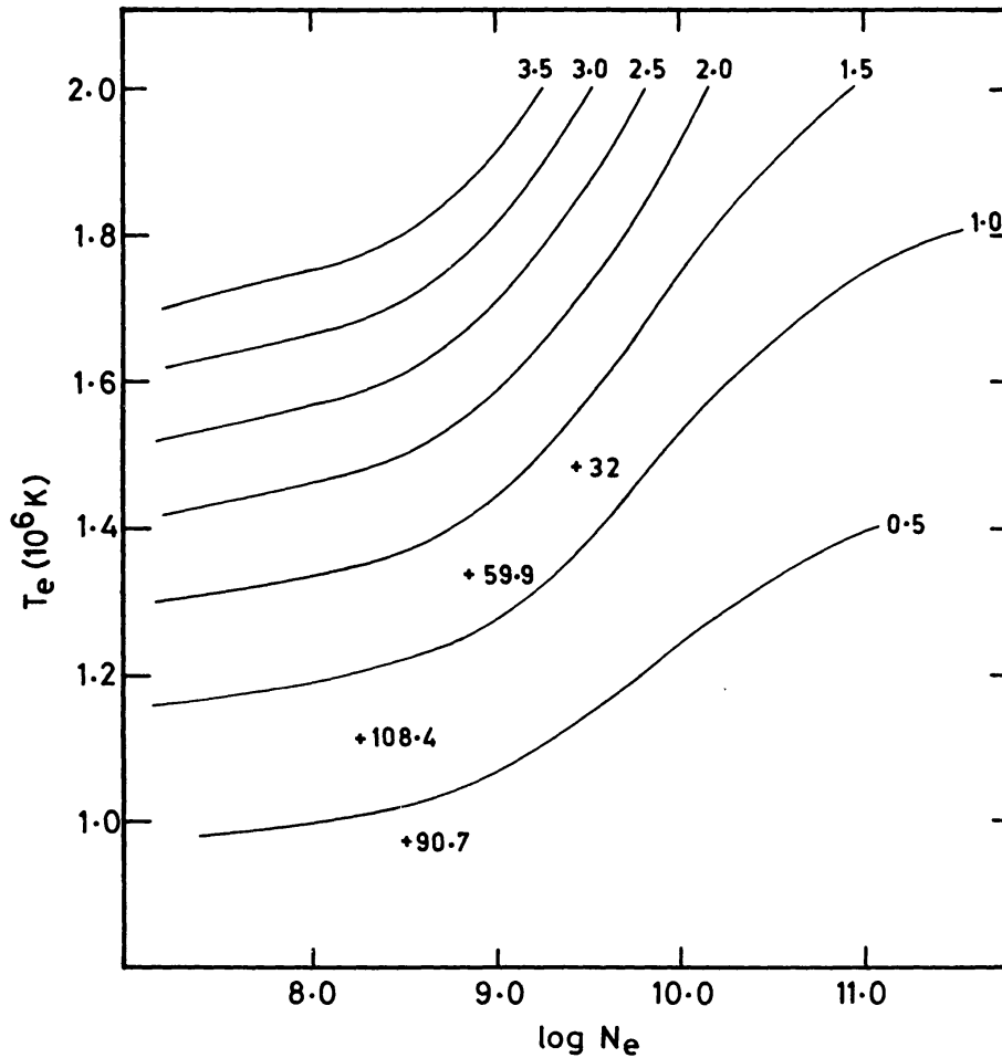
Figure 5. Contours of equal ratios of [\text{Fe XI}] 7892/[\text{Fe X}] 6374 plotted in (T_e, \log N_e) plane. The observed ratios plotted against the assumed densities, indicate the temperature.
