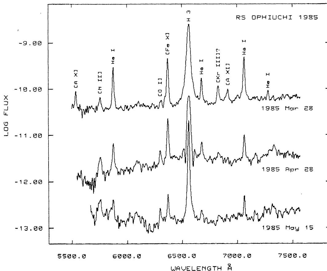
Figure 2. Spectra of RS Oph on days 60, 91, and 108, in the range 5600–7500 Å. H\alpha was overexposed on April 28. Instrumental response correction on May 15 is uncertain shortward of 6200 Å. Note the fading of coronal and He I lines, and brightening of [O I] and [N II] lines. Flux is in units of \text{erg cm}^{-2} \text{s}^{-1} \text{Å}^{-1} . Top two spectra are shifted upwards by three and one unit respectively in log (flux).
