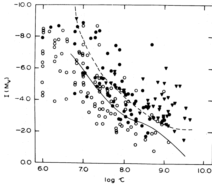
Figure 6. The I(M_V) -log age diagram along with the theoretical dependences obtained in the present work. The dashed curve represents the theoretical curve calculated for the whole cluster and the continuous curve represents the curve calculated for the main sequence part of the cluster.
