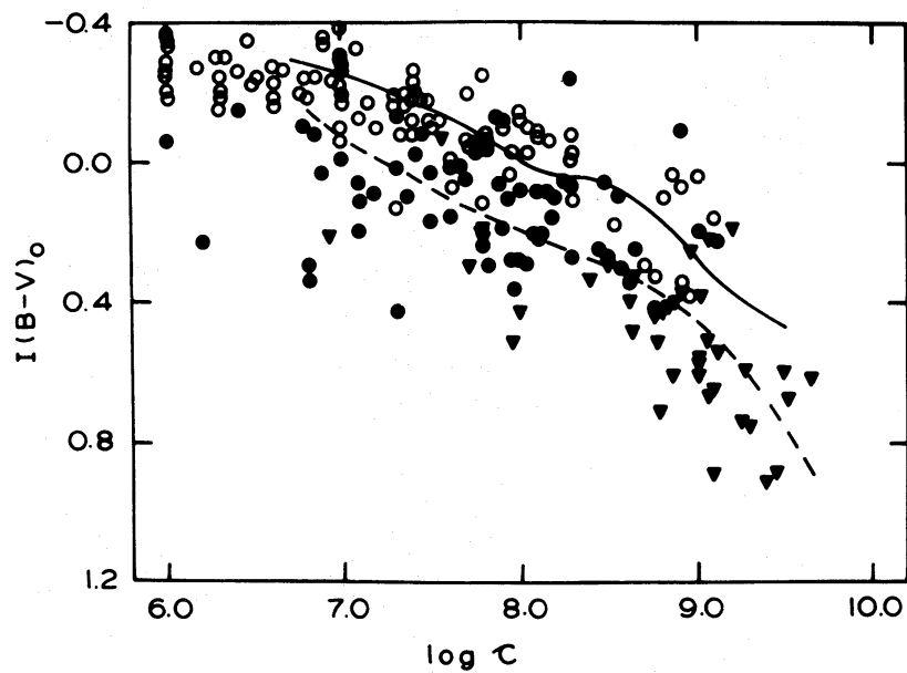
Figure 9. The I(B-V)_0 -log age diagram. The curves and symbols are the same as in Figs 6 and 1, respectively.
