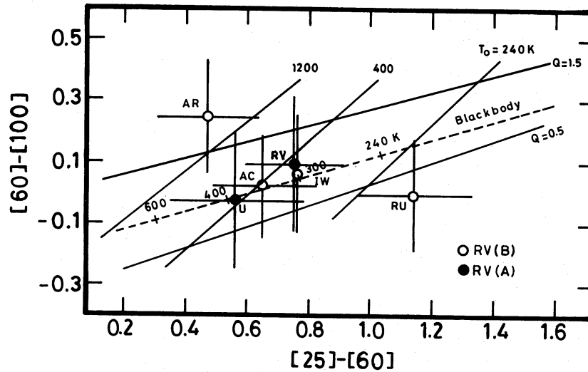
Figure 2. Plot of the [60]-[100] colours of RV Tauri stars against their [25]-[60] colours after normalizing as indicated in Beichman et al. (1985b). The solid lines represent the loci for constant inner-shell temperature and the quantity Q . The dashed line shows the locus for a blackbody distribution.
