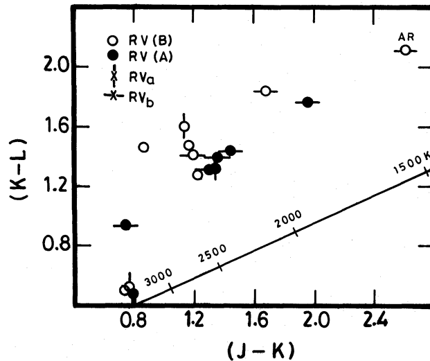
Figure 3. Plot of (K-L) colours of RV Tauri stars detected by IRAS against their corresponding (J-K) colours. The position of AR Pup is indicated. The three objects lying close to the blackbody line are AC Her, RU Cen and R Sct.
