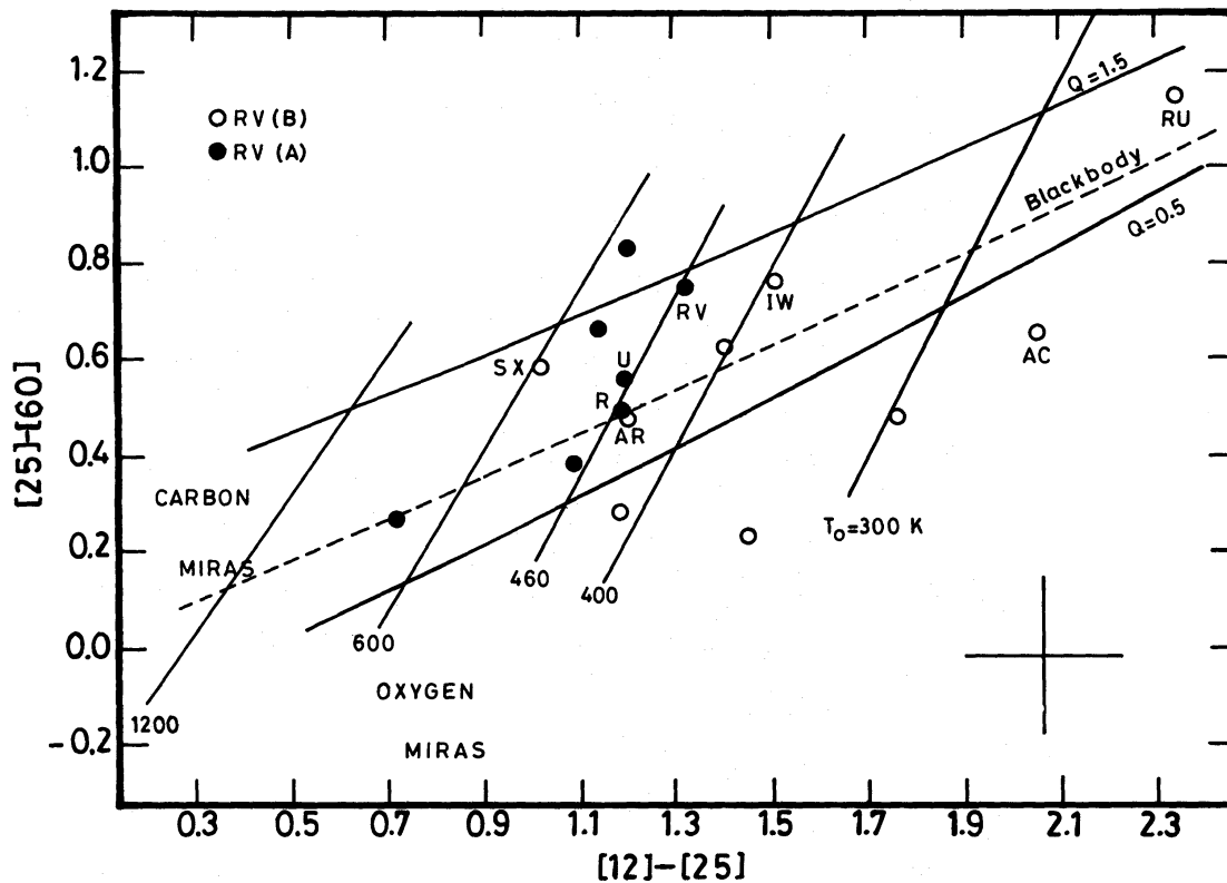
Figure 1. Plot of [25]-[60] colours of RV Tauri stars against their [12]-[25] colours after normalizing as indicated in Beichman et al. (1985b). Some of the objects are identified by their variable-star names. Typical error bars are shown in the bottom right hand corner. The lines represent the loci for constant inner-shell temperature and the quantity Q . Note the separation of group A and B stars at T_0 \sim 460 K. Positions occupied by a sample of carbon and oxygen Miras are also shown. The Q = 1.0 line differs from the blackbody line by a maximum of \sim 0.05 .
