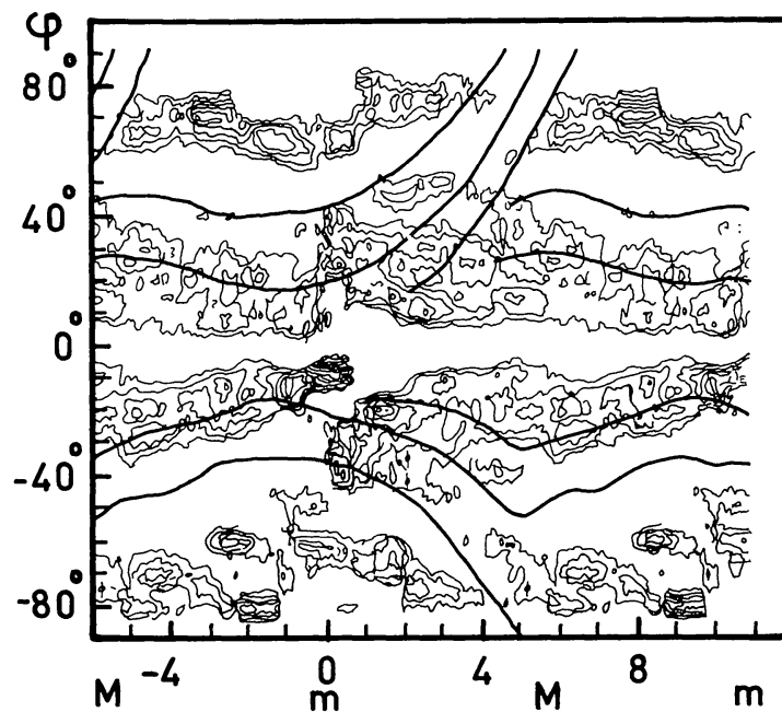
Fig. 5. The map of isovalues of the quantity \sigma_{5303} - \bar{\sigma}_{5303} , (Leroy and Noens, 1983). \sigma_{5303} is the standard deviation of coronal intensity at each latitude over periods of about 1 year and \bar{\sigma}_{5303} is the latitude average of \sigma_{5303} over 20^\circ intervals. Leroy and Noens (1983) have used the mean of the three values of \sigma_{5303} from identical phases of the cycles 18, 19, and 20 (1944–1974) to represent a typical average cycle. The thick lines are the migration trajectories of neutral filament bands for cycle 20 (Makarov, Leroy, and Noens, 1987). m – minimum epoch of solar cycle. M – Maximum epoch of solar cycle. Ordinate – solar latitude in degrees.
