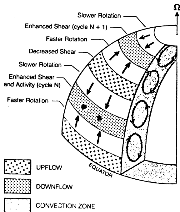
Fig. 7. Schematic diagram showing the surface motions, zones of enhanced and decreased shear at solar maximum for cycle N (sunspots in active zone) along with the emergence at high latitude of cycle N + 1 . The bands on the surface indicate the various predicted large scale motions produced by the rolls shown as ovals in the convection zone (not needed for the discussions in this paper). (Reproduction of Figure 3 of Snodgrass (1987a). By courtesy of H. B. Snodgrass and the Astrophysical Journal .)
