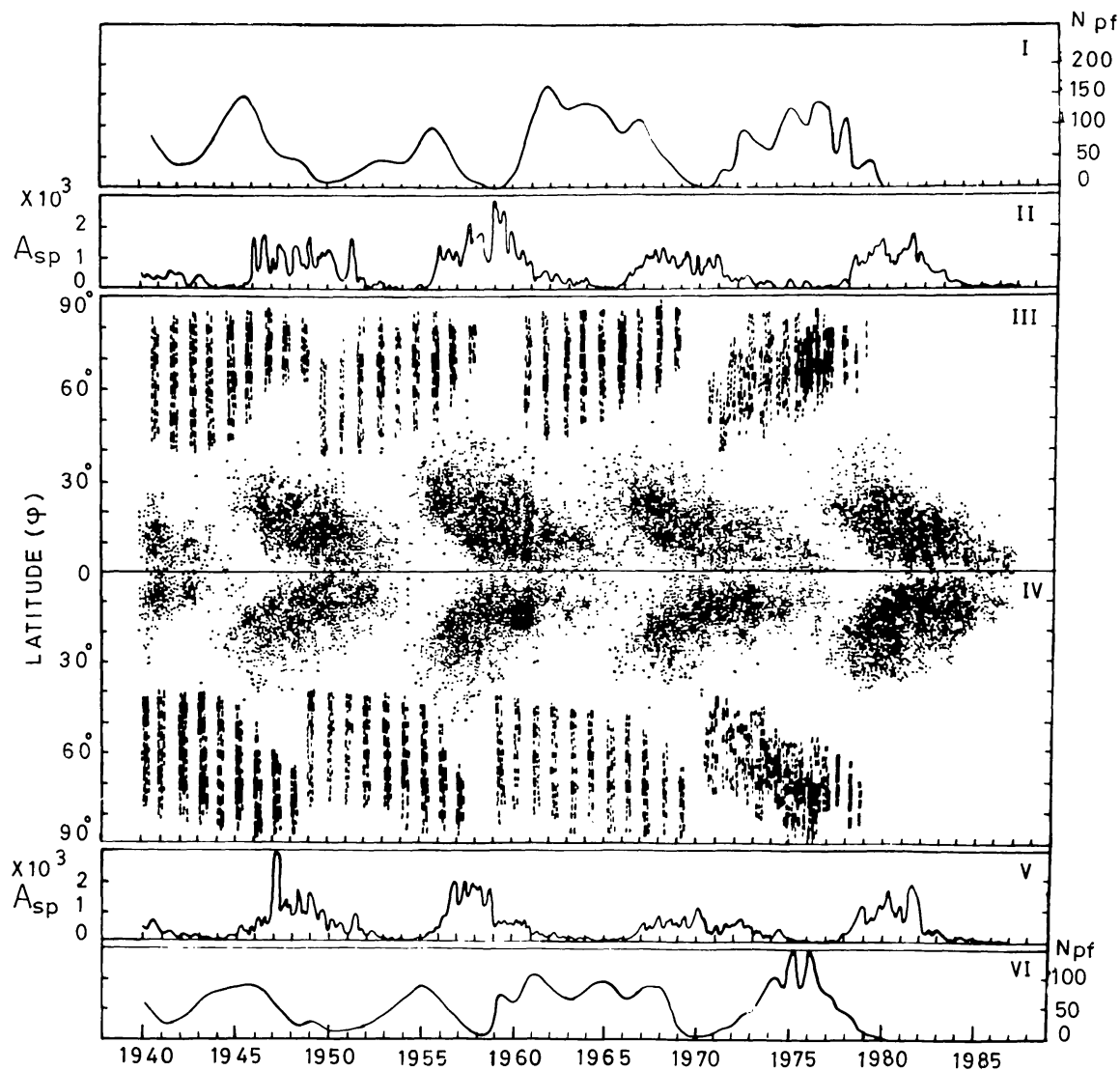
Fig. 4. Boxes III and IV show the latitude distribution of polar faculae and sunspots (butterfly diagram) during 1940–1985. Notice that the faculae make their appearance first between 40^\circ – 70^\circ latitudes in the northern and southern hemispheres and then migrate towards the respective poles as the cycle advances. The superposed lines are the migration trajectories of filaments reproduced from Figure 1 after smoothing to show the epochs of polar reversals. Notice that the polar faculae make their appearance immediately after every polar reversal. Boxes II and V are the sunspot areas A(\text{Sp}) for these years as in Figure 1. Boxes I and VI: the continuous line represents the polar faculae counts ( N_{pf} ) in the northern and southern hemispheres.
