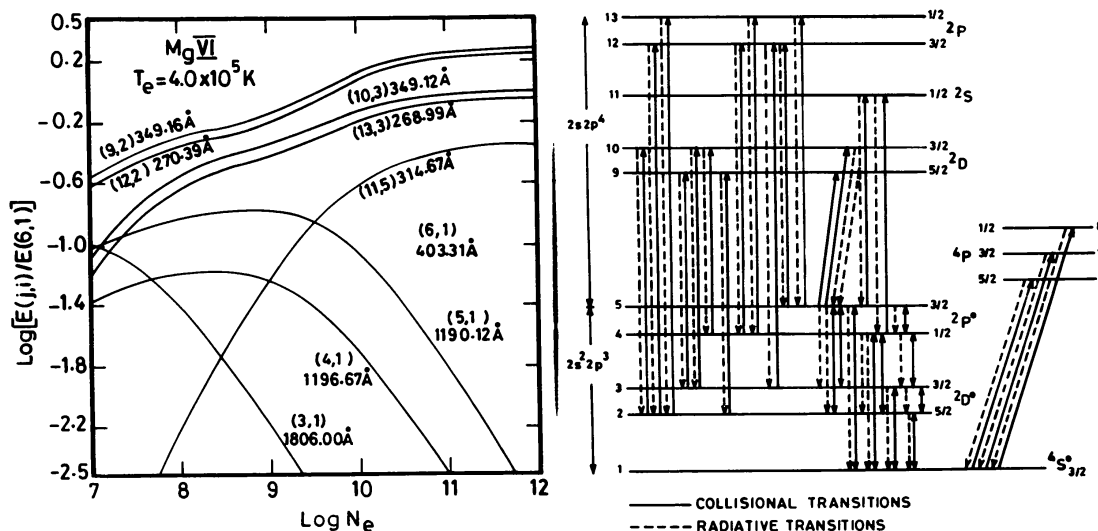
Fig.1. Line intensity ratios E(j,i)/E(6,1) as a function of electron density N_e . T_e is the temperature for maximum relative ion abundance for Mg VI.
