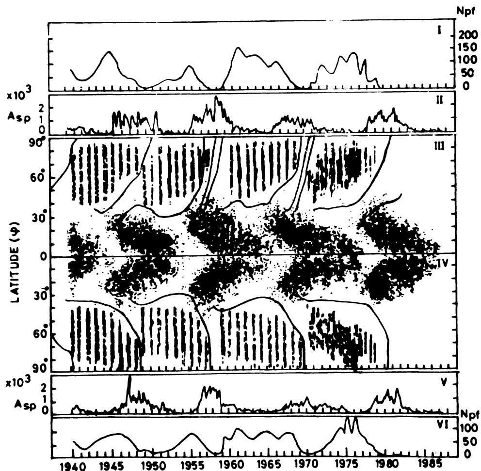
Figure 4. Boxes III and IV show the latitude distribution of polar faculae and sunspots (butterfly diagram) during 1940–1985. The superposed lines are the migration trajectories of filaments reproduced from Figure 1 after smoothing, to show the epochs of polar reversals. Boxes II and V show the sunspot areas A_{sp} as in Figure 1. Boxes I and VI show the counts ( N_{pf} ) of polar faculae in the north and south hemispheres.
