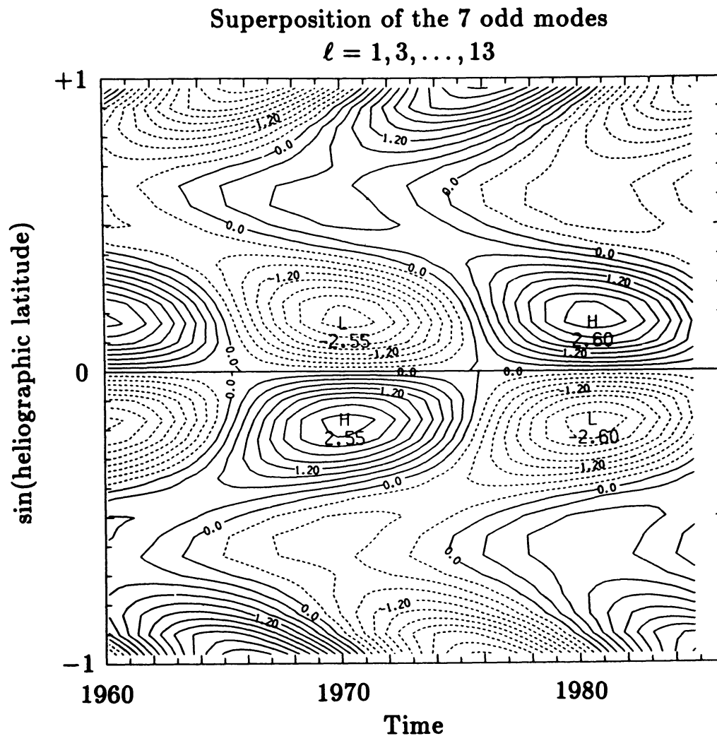
Figure 5. Synthetic evolutionary diagram computed as the superposition of 7 discrete harmonic modes (with purely sinusoidal time variations), with only odd values of l ( l = 1, 3, \dots, 13 ). (Reproduction of Fig. 4 of Stenflo (1988). By courtesy of Stenflo and Kluwer Academic Publishers.)
