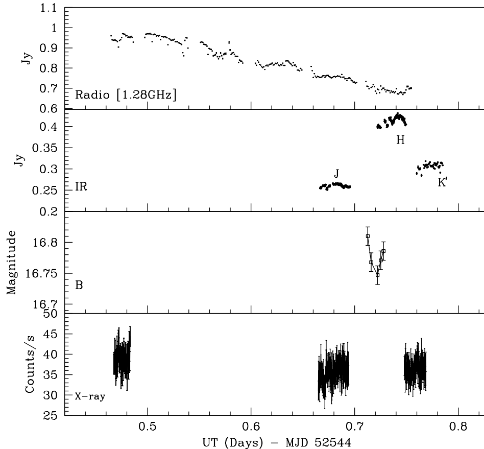
Figure 4. Light curves of SS 433 on the 2002 September 27, as obtained by our multi-wavelength campaign at different wavelengths. Upper panel: radio observation at 1.28 GHz at GMRT, Pune. Second panel: IR observation at J , H and K' bands at Mt. Abu. Third panel: B -band observation at the State Observatory, Nainital. Last panel: background subtracted X-ray count rates by the RXTE satellite.
