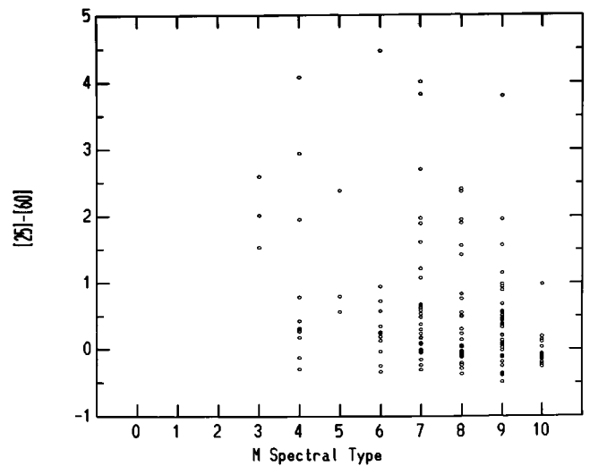
Fig. 10. [25]–[60] colour of IRAS unidentified sources which have best-quality flux density data in both these wavelength bands vs. their spectral type
