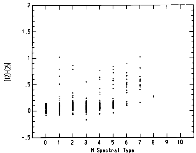
Fig. 6. Similar data as in Fig. 5 for BSC M giants
