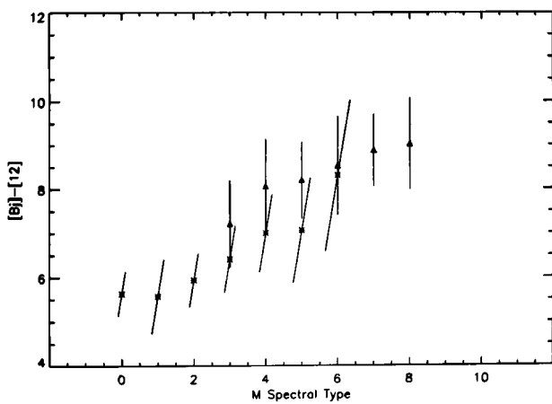
Fig. 4. Mean B_j -[12] colours of IRAS unidentified sources and of BSC giants as a function of M spectral type. The symbols “delta” and “*” refer to IRAS unidentified sources and BSC giants, respectively. The error bars shown on the data points correspond to the rms deviations of the colours from their mean values. The error bars on the mean colours of the BSC stars are shown slanted to avoid overlaps
