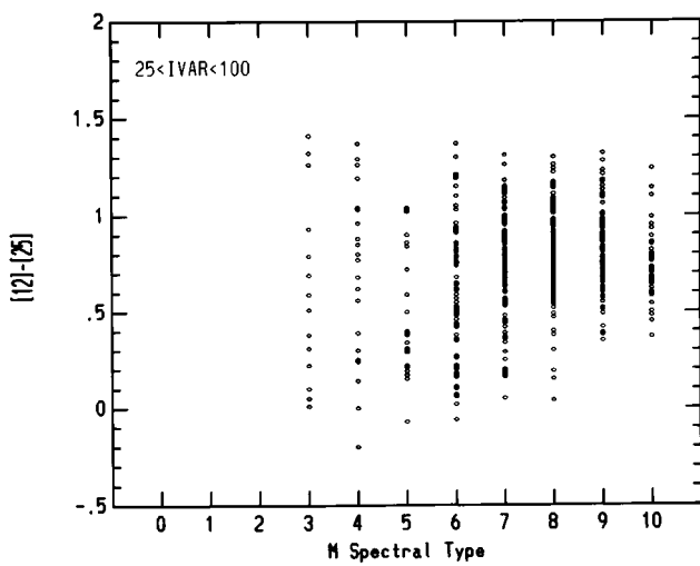
Fig. 9. [12]–[25] colour vs. M spectral type of unidentified IRAS sources with quality-3 flux densities at both 12 \mu\text{m} and 25 \mu\text{m} and whose variability index IVAR is > 25
