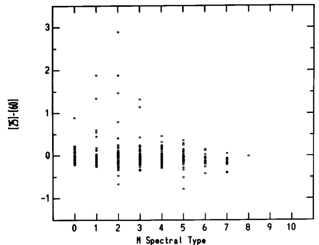
Fig. 11. Similar data as in Fig. 10 for BSC giants
