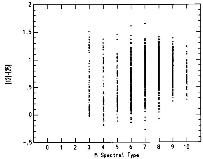
Fig. 5. [12]-[25] colour of IRAS unidentified sources which have best-quality flux density data vs. their M spectral type
