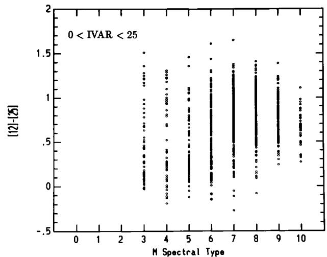
Fig. 8. [12]-[25] colour vs. M spectral type of unidentified IRAS sources with quality-3 flux densities at both 12 \mu\text{m} and 25 \mu\text{m} and whose variability index IVAR is < 25
