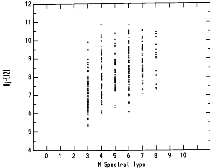
Fig. 2. B_j-[12] colour vs. spectral type of unidentified IRAS sources with best-quality flux density data at only 12\ \mu\text{m} (which could be associated with optical counterparts) on the SERC plates by searching the Guide Star Catalog (Version 1). The optical object (when it was the only one) on the SERC plates within a circle of radius 15'' from the IRAS source position was considered as its optical counterpart. The B_j magnitudes are from GSC Version 1
