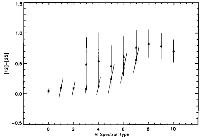
Fig. 7. Mean [12]-[25] colours of IRAS unidentified sources and BSC giants vs. M spectral type. The symbols “delta” and “*” have the same meanings as in Fig. 4. The error bars shown on the data points correspond to the rms deviations of the colours from their mean values. The error bars on the mean colours of the BSC stars are shown slanted to avoid overlaps
