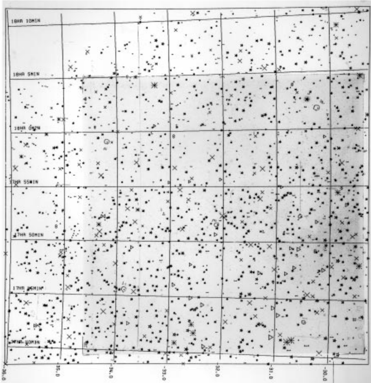
Fig. 1. Reduced-scale version of a I-N objective prism spectrum plate obtained at a dispersion of 3400 \text{ \AA mm}^{-1} with the Curtis Schmidt Camera at CTIO, Chile. The deepest plates reach I \sim 13.5 . Each plate covers 5^\circ \times 5^\circ . The plate scale is 96''.6 \text{ mm}^{-1} . The different symbols on the photographic print refer to IRAS sources with F_\nu(12 \mu\text{m}) \geq F_\nu(25 \mu\text{m}) . The size of the symbol is proportional to F_\nu(12 \mu\text{m}) . These symbols refer to sources as listed below: 1 = 1000, star = 1100, x = 1110, * = 1111, triangle = 1101, x with bar on top = 1010, x with bar top/bottom = 1011, infinity = 1001. The four numbers on the right of the sign “=” refer in the order to the flux density of these sources at 12, 25, 60 and 100 \mu\text{m} respectively, where “0” means flux density is below the detection threshold and “1” means flux density is above it
