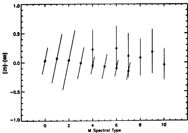
Fig. 12. Mean [25]-[60] colours of unidentified IRAS sources and BSC giants vs. M spectral type. The symbols “delta” and “*” have the same meanings as in Fig. 4. A large number of sources have [25]-[60] colours which deviate by a very large margin from their mean values (see Fig. 10). The mean [25]-[60] colours (shown in this figure) of the IRAS unidentified sources are therefore limited to only those sources whose [25]-[60] colour is \leq 1.0 . Mean colours of stars with spectral types numbering \leq 5 are not shown in the figure as they are not statistically significant. The error bars shown on the data points correspond to the rms deviations of the colours from their mean values. The error bars on the mean colours of the BSC stars are shown slanted to avoid overlaps
