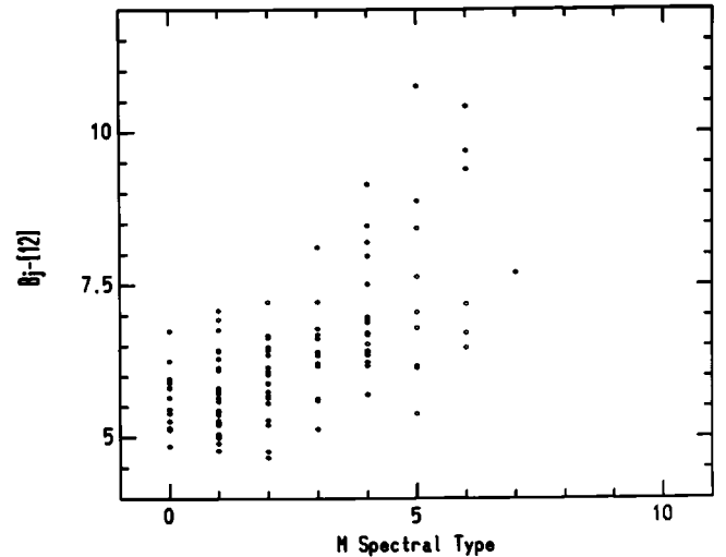
Fig. 3. Similar data as in Fig. 2 for BSC M giants. However, the BSC giants have IRAS quality-3 flux density data in the three bands 12 , 25 , and 60\ \mu\text{m} unlike the IRAS unidentified sources with which they are being compared
