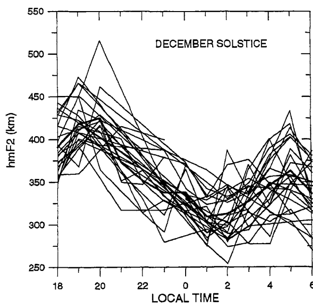
Figure 2. Nocturnal variation of the height of F2 layer peak density ( h_{\max} ) at Cachoeira Paulista during the December solstice. The thick line shows the variation of mean h_{\max} .
