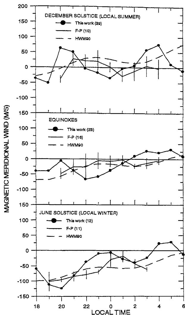
Figure 1. Nocturnal variation of neutral wind in the magnetic meridian (positive equatorward) over Cachoeira Paulista for the December (D), equinox (E), and June (J) months of high solar flux conditions. The HWM90 model winds and winds from FPI measurements at the same location (not simultaneous) are also shown for comparison. The number of nights of data are also shown both for ionosonde and FPI winds. The average solar 10.7 cm flux for the D, E and J months is 196.2, 194.7 and 185.3 units, respectively.
