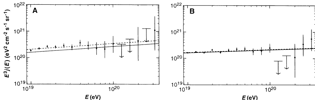
Fig. 1. Maximum L fits of the pure power law model 1 over the energy range 10^{18.95} eV \leq E \leq 10^{20.55} eV. We fitted the effective flux (dashed lines) that results from the real differential flux (solid lines) by taking the experimental energy resolution into account. The data are given as 68% C.L. error bars or as 84% C.L. upper limits. For illustration purposes we multiplied the steeply falling flux by E^3 . (A) Fit to the combined Fly's Eye monocular, Akeno, and Haverah Park data with \approx 30\% energy resolution, corresponding to an L significance of 39% above 10^{20} eV. (B) A typical example resulting from "data" simulated for a quadrupled exposure with 10% energy resolution. For these data, model 1 would be ruled out at the 99% C.L.
