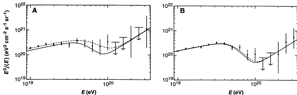
Fig. 2. Same as Fig. 1 but for the exotic model 5. In contrast to the pure power law model 1, the L significance above 10^{20} eV [82 and 60% in the case of (A) and (B), respectively] typically stays within the 1\sigma level for both exposures.
