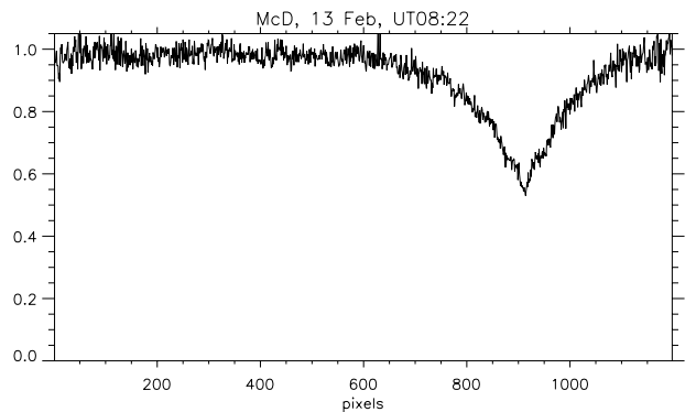
Fig. 7. Spectrum from McD. The order containing H\alpha . Again low counts due to high resolution. The throughput was measured to be only \sim 1.7\%
