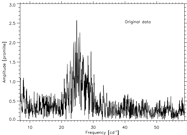
Fig. 8. Amplitude spectrum of the full H\alpha line-index data set. The oscillation modes are clearly visible, although they are not well resolved.
