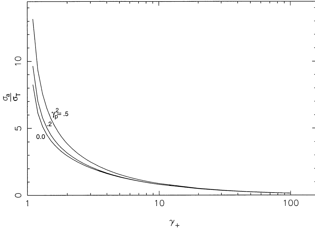
Figure 9. Variation of the total cross section \sigma_a for pair annihilation with the positron energy \gamma_+ for different values of the plasma density parameter \gamma_p^2 .
