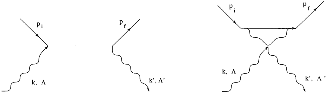
Figure 1. The direct and exchange diagrams for Compton scattering: e^- + \gamma \rightarrow \gamma' + e^- .
