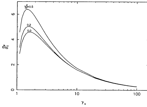
Figure 11. Variation of the pair production cross section \sigma_p with positron energy \gamma_+ for different values of the plasma density parameter \gamma_p^2 .
