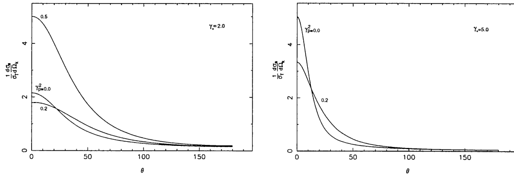
Figure 8. Variation of the differential cross section for pair annihilation with the angle \theta between the positron beam and the photon ( \gamma_1 ) for different positron energies \gamma_+ and plasma density parameters \gamma_p^2 .
