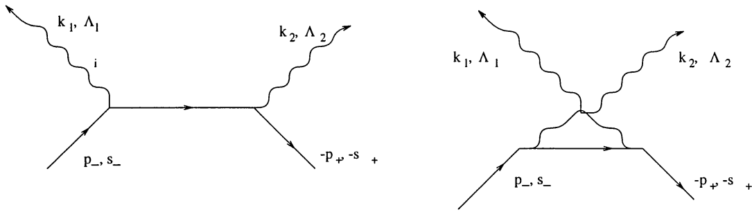
Figure 6. Direct and exchange diagrams for electron-positron annihilation : e^- + e^+ \rightarrow \gamma_1 + \gamma_2 .
