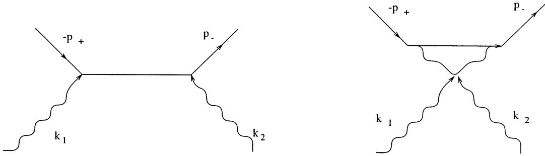
Figure 10. Feynman diagrams for pair production.
