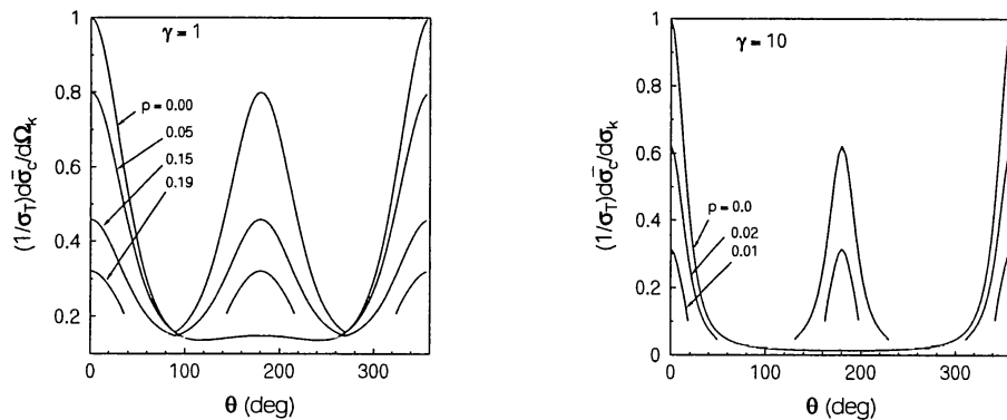
Figure 4. Variation of the differential cross section for Compton scattering with the scattering angle \theta for different values of the plasma density parameter p , the initial photon energy \gamma , and the final photon energy \gamma' corresponding to the first root of Eqn. (3).
