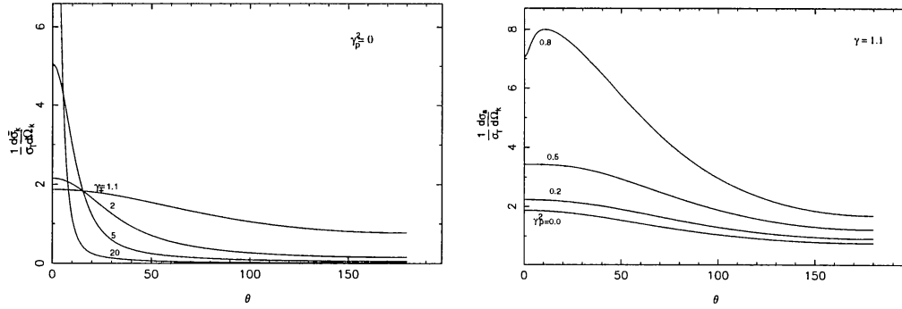
Figure 7. Variation of the differential cross section for pair annihilation with the angle \theta between the positron beam and the photon ( \gamma_1 ) for different positron energies \gamma_+ and plasma density parameters \gamma_p^2 .
