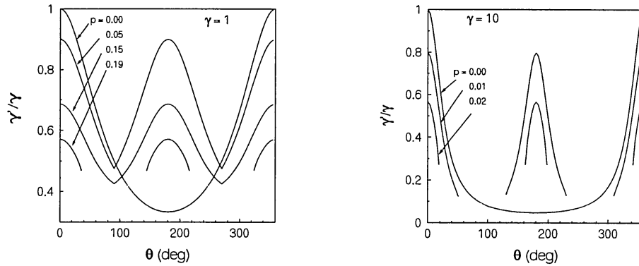
Figure 2. Variation of the first root ( \gamma'/\gamma ) of Eqn. (3) vs. the scattering angle \theta for different values of the plasma density parameter p and initial photon energy \gamma .
