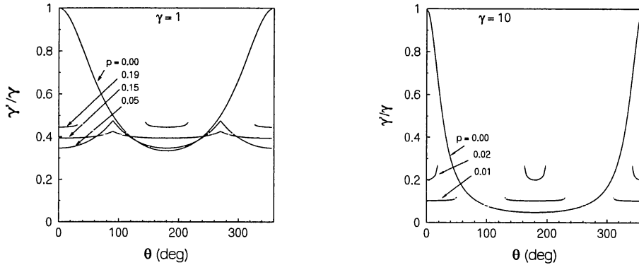
Figure 3. Variation of the second root ( \gamma'/\gamma ) of Eqn. (3) vs. the scattering angle \theta for different values of the plasma density parameter p and initial photon energy \gamma .
