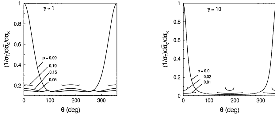
Figure 5. Variation of the differential cross section for Compton scattering with the scattering angle \theta for different values of the plasma density parameter p , the initial photon energy \gamma , and the final photon energy \gamma' corresponding to the second root of Eqn. (3).
