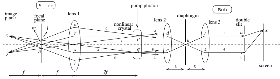
Figure 1. Light produced in a nonlinear crystal via spontaneous parametric downconversion (SPDC) is shared by Alice and Bob. By observing her photons at the focal or image plane of her lens, Alice leaves Bob's photons, respectively, as a wave-like object with a definite momentum, or a particle-like object with a definite point of origin. Access to Bob's interferometer is restricted to horizontal modes, by means of two juxtaposed lenses with an intervening diaphragm perforated at the shared focus.
