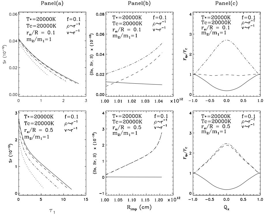
Fig. 5. The ray source functions versus the optical depths along the ray for \frac{r_e}{R} = 0.1, 0.5 . Continuous line for ray 1, dashed line for ray 6, dashed-dotted for ray 12 and dotted line for ray 18 are given above. Panel a ) v_a = 0, v_b = 0 , Panel b ) shows the source functions versus R_{\text{imp}} plotted for \frac{r_e}{R} = 0.1, 0.5 Source functions for self radiation continuous line ( S_s ), distorted for different source function dashed line of the distorted atmosphere ( S_r ), total source function ( S ) dashed-dot. Panel c ) shows the normalized fluxes \frac{F_{Q_x}}{F_c} against Q_x where F_c is the flux in the continuum and Q_x = \frac{x}{x_{\text{max}}} (see Fig. 4 for the definition of x ). Fluxes due to self radiation are shown by the continuous line, those due to distorted source function by dashed line, and those due to total source function by the dashed dot.
