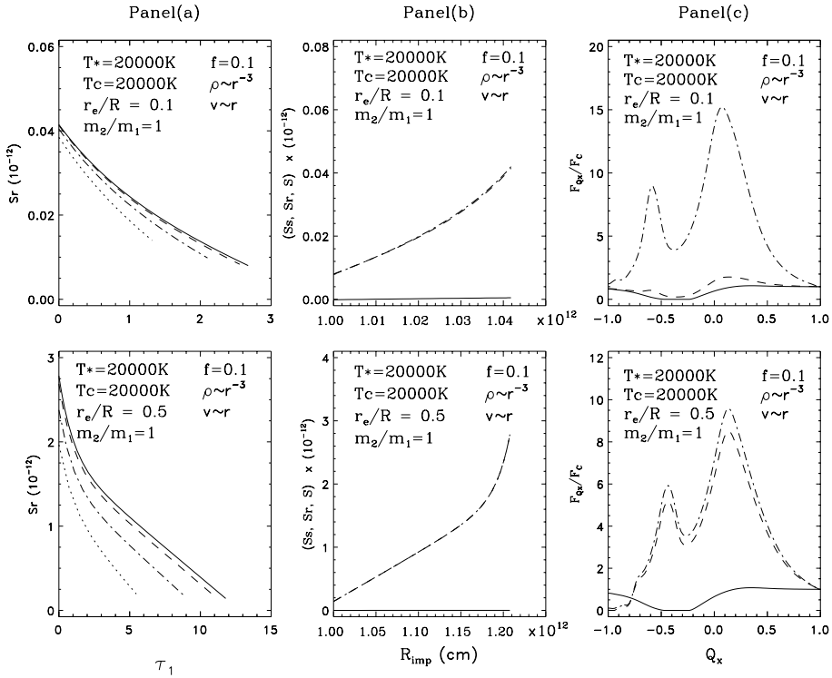
Fig. 6. Same as Fig. 5 but with v_a = 0 and v_b = 10 mtu (mean thermal units).
