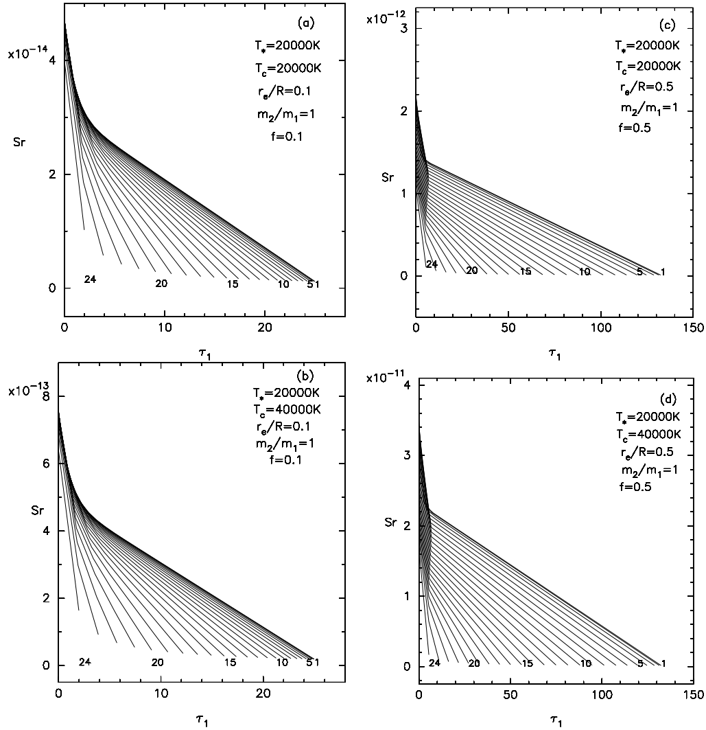
Fig. 3. The source functions are plotted against the optical depths \tau_1 's measured along the rays such as A_1JKL, \dots, DEFG . The curve labeled 1 corresponds to the ray A_1JKL, \dots , the curve labeled 2 to the ray DEFG, \dots
