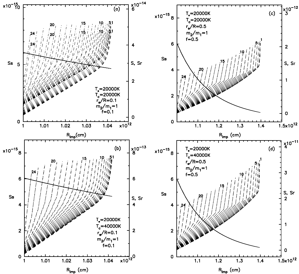
Fig. 2. Source functions along the rays inside the distorted surface with respect to the distances along the axes OA_1 . R_{imp} represents the values OA_1, OJ, OK, \dots . We have given an irradiation proportional to (T_c/T_*)^4 where T_* is the temperature of the primary with centres at O and T_c is the temperature of the star at B (see Fig. 1). The density varies as r^{-3} . The source functions S_s , for the self radiation are shown through the solid line with the scale given on the left side of the graph while those representing the ray source functions S_r are shown by the dashed lines with its scale given on the right side of the graph. The combined source function S (= S_s + S_r) are shown by the dashed-dot curves with its scale given on the right side of the graph. The numbers given in these figures such 1, 5, 10, 15, 20, 24 represent the rays such as A_1C, DI, PV, \dots . The S 's are plotted against the distances R_{imp} = A_1O, JO, KO, \dots . The ray corresponding to A_1C is labeled as 1 and that corresponding to DI as 2 and so on.
