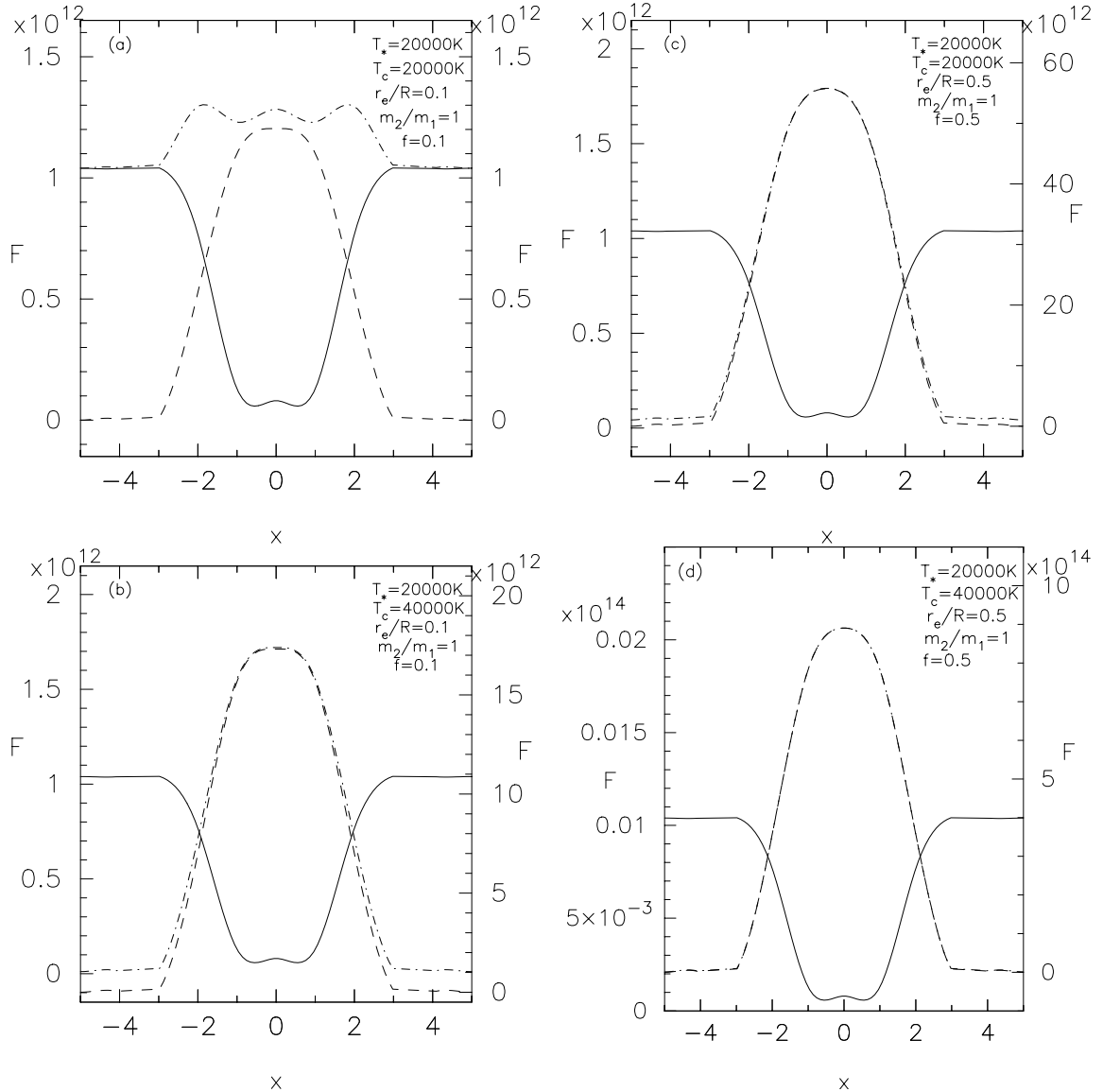
Fig. 4. The flux profiles are plotted against frequency measured in units of Doppler width x , (where x = \frac{(\nu - \nu_0)}{\Delta\nu_D} , \nu and \nu_0 being the frequencies in the line and at the centre of the line and \Delta\nu_D is the Doppler width) for \rho \sim r^{-3} .
