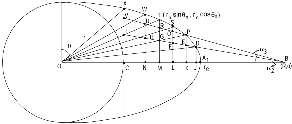
Fig. 1. Schematic diagram of the distorted atmosphere of the component.
