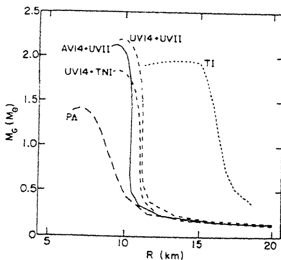
Figure 8. The mass-radius relation for neutron stars (from Wiringa, Fiks, Fabrocini 1988).
