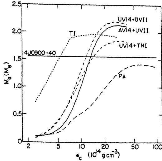
Figure 7. Gravitational mass versus central density. The modern equations of state predict maximum mass \sim 2 M_{\odot} , while the very soft equation of state (PA) predicts a maximum mass \leq 1.5 M_{\odot} . The horizontal line is the estimated mass of the neutron star in the x-ray binary 4U0900-40 (from Wiringa, Fiks, Fabrocini 1988).
