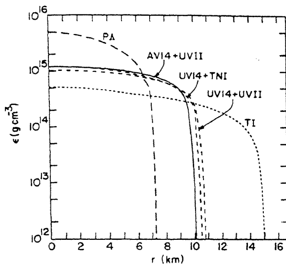
Figure 6. Density profiles of a 1.4M_{\odot} neutron star calculated with various equations of state. In addition to the three modern equations of state which include 3-body forces, the figure also shows the density profile corresponding to a very soft equation of state (PA) and a very stiff equation of state (TI). All the three modern models predict a radius for the star \approx 10.5\text{ km} , and a central density \sim 6\rho_0 . The crust is only \sim 1\text{ km} thick in these models (from Wiringa, Fiks, Fabrocini 1988).
