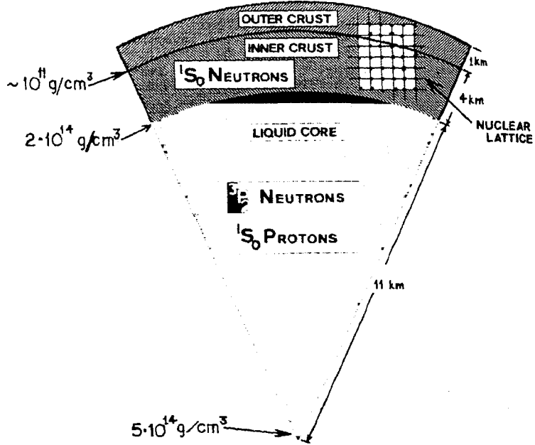
Figure 2. A schematic cross-section of a 1.4M_{\odot} neutron star based upon a stiff equation of state (from Sauls, 1989).
