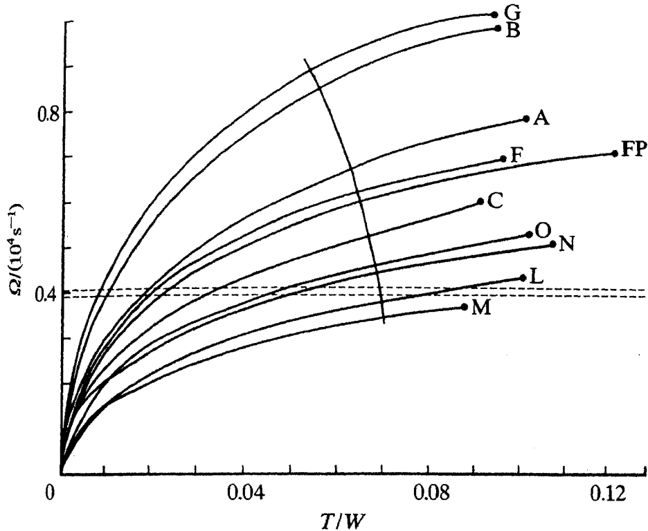
Figure 11. Sequences of uniformly rotating neutron stars of baryon masses M_B = 1.4M_\odot for various equations of state. The angular velocity \Omega is plotted against T/|W| , the ratio of rotational energy to the potential energy of rotating stars. The termination point of each sequence corresponds to \Omega = \Omega_K . The diagonal line crossing the sequences is a conservative estimate of the smallest rotation rate for which the model could be unstable to non-axisymmetric perturbations. The horizontal dashed lines are the angular velocities of the two fastest pulsars: PSR 1937+214 (upper line) and PSR 1957+20 (lower line). The main conclusion is that only the stiff equations of state (L, M, N and O) are consistent with a mass of 1.4M_\odot and the observed periods of these pulsars (from Friedman and Ipser 1992).
