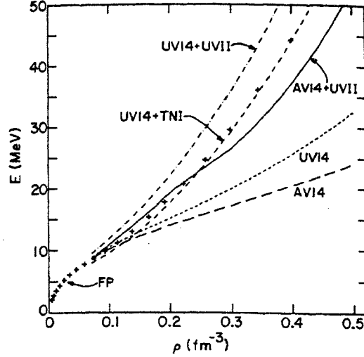
Figure 5. Energy per nucleon versus baryon density with and without 3-body forces in pure neutron matter. UVI4 and AVI4 use only 2-body forces, while the curves with the additional labels UVII and TNI include 3-body forces (from Wiringa, Fiks, Fabrocini 1988).
