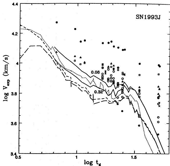
Fig. 5. Variation of velocities of different absorption lines observed in the spectra of SN 1993J as a function of time since outburst. Filled circles: H\alpha ; open squares: H\beta , H\gamma ; open triangles: He I lines; open circles: Fe II lines; crosses: Ca II and O I lines; stars: Ba II and Sc II lines. The continuous lines denote photometric velocities derived from the radii estimated by us for the two values of E(B - V) as marked. The dotted line is based on radii determined by Lewis et al. (1994) for an A_v = 0.58 . The short-dashed lines and the long-dashed lines are based on the blackbody fits of Richmond et al. (1994) for E(B - V) = 0.08 and 0.32 respectively
