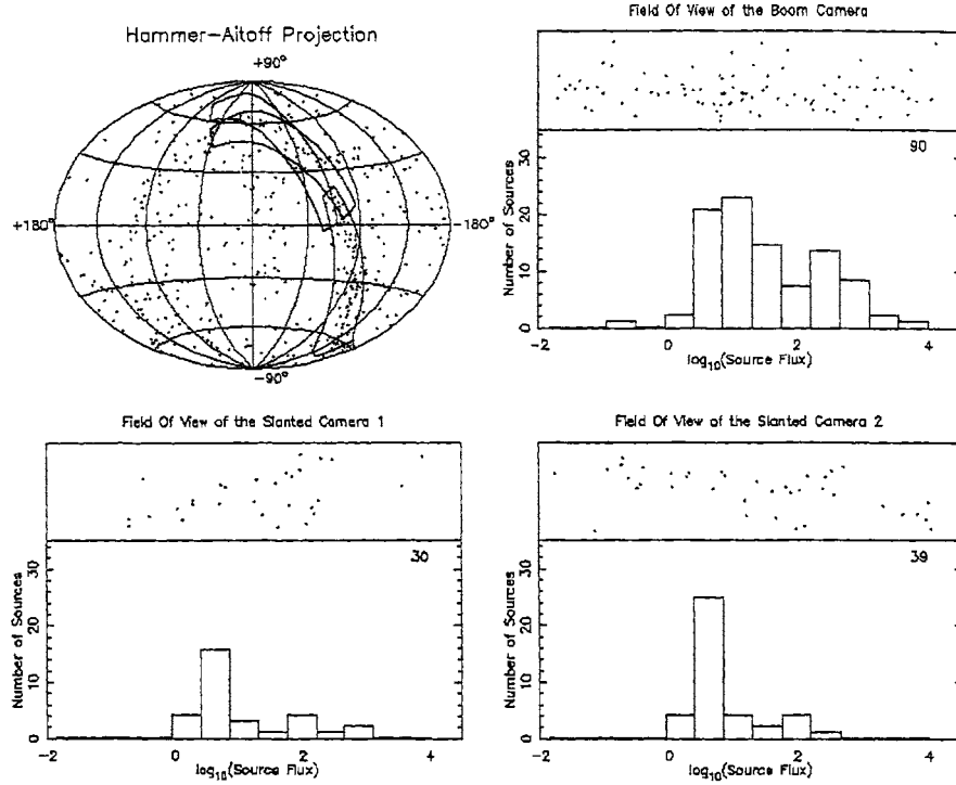
Figure 1. A snapshot of the simulation. The first panel shows the sky distribution of X-ray sources and the fields of view of the three SSM cameras. The other panels show the source distribution in the three camera FOVs, the number of such sources and their flux distribution histogram.
