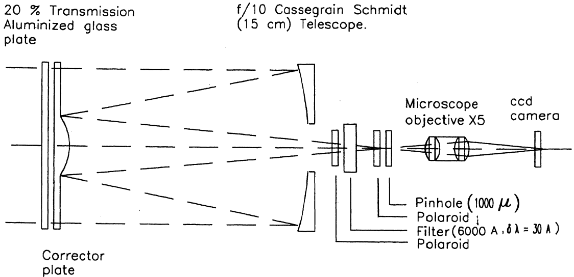
Figure 1 : Schematic layout of the instrument.
