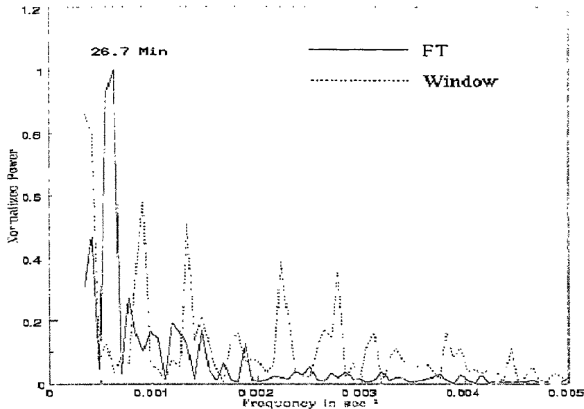
Figure 4. Plot of frequency of intensity of AR and normalized power.
