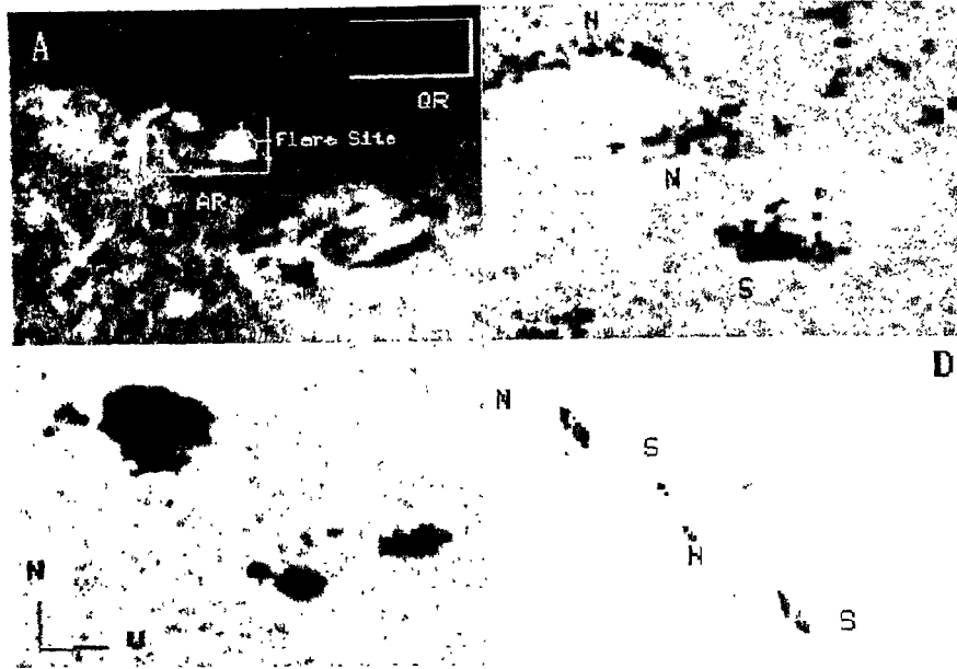
Figure 1. Figure 1A Shows the location of AR NOAA 9033 and Quiet Region (QR) used in the analysis, Figure 1B Shows SOHO/MDI magnetogram images of NOAA 9033 at 01:36 UT, Figure 1C shows SOHO/MDI continuum images of NOAA 9033 at 01:36 UT and Figure 1D Shows the quadrupolar reconnection scenario for the origin of homologous flares proposed by Machado et al.(1983).
