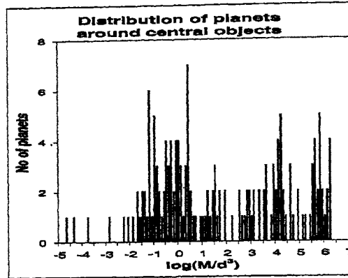
Figure 3. M_*/(\text{Planet Distance})^3 distribution of planets outside the solar system and solar system objects
