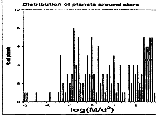
Figure 2. M_{star}/(\text{Planet Distance})^2 distribution of extra-solar-system planets and solar system objects.
