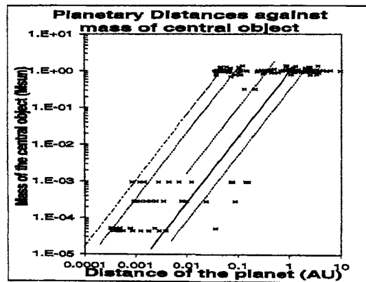
Figure 1. Distance distribution of planets outside the solar system. \times indicates extra-solar-system planets and moons of solar system objects. \circ indicates the solar system planets.
